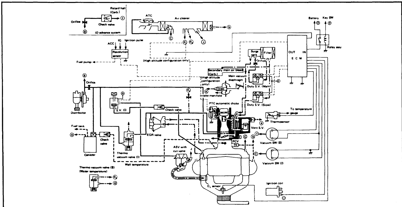
Fig. 2: Subaru Vacuum Diagram
