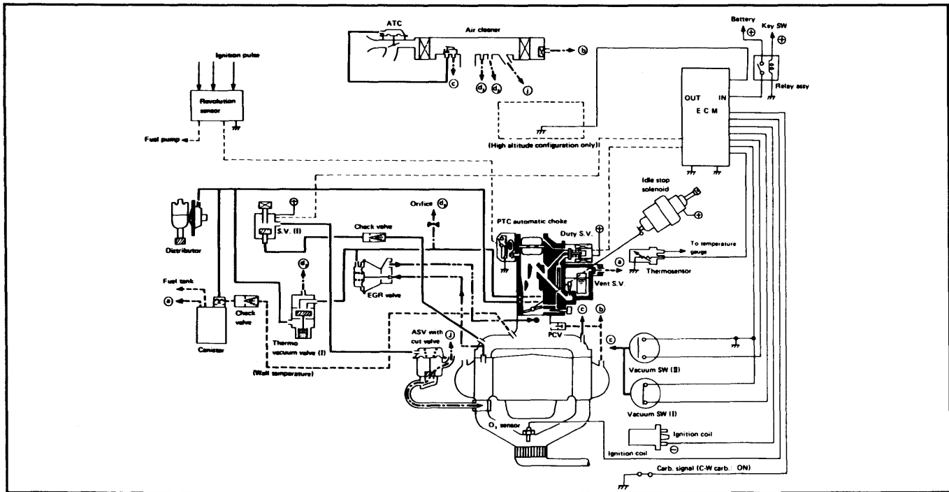
Fig. 1: Subaru Vacuum Diagram
