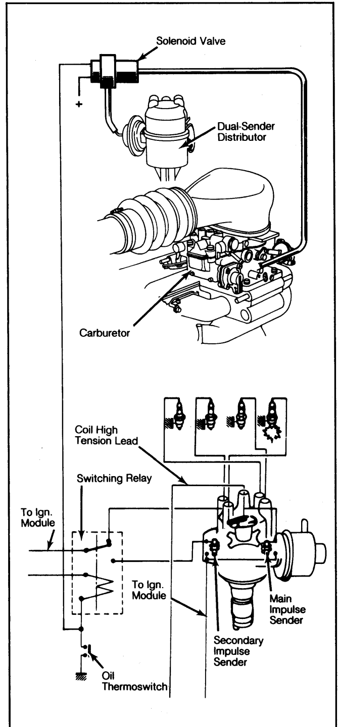
Fig. 1: Le Car Vacuum Advance Correction System
