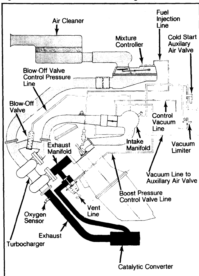
Fig. 3: Porsche 924 Turbo Vacuum Diagram
