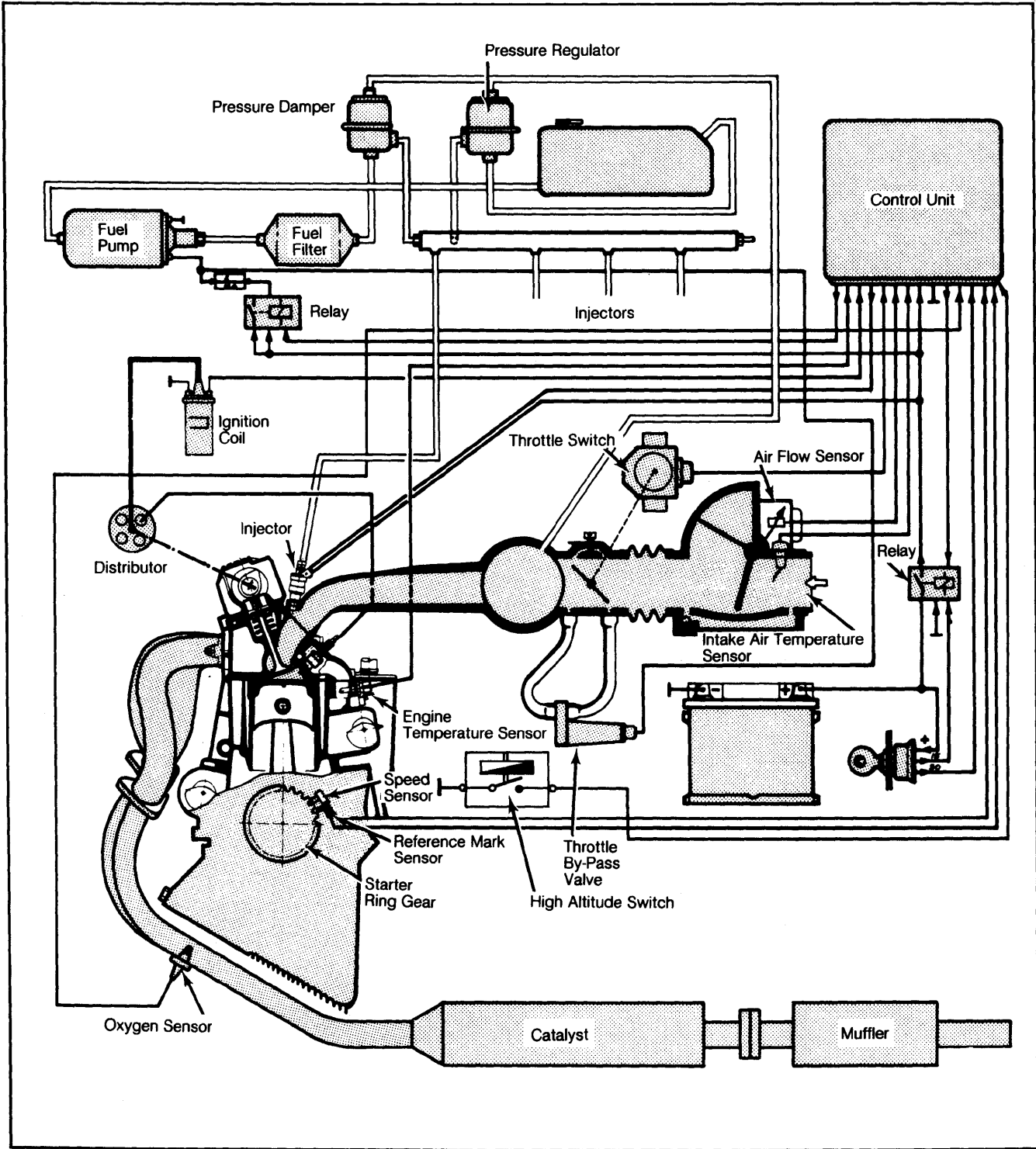
Fig: 5 Porsche 944 Exhaust Emission System
