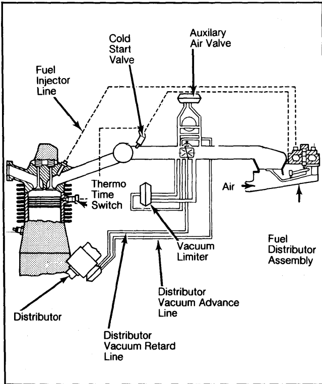
Fig. 1: Porsche 911SC Vacuum Diagram
