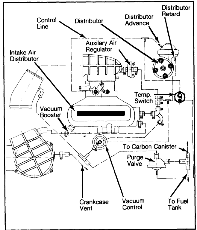
Fig. 4: Porsche 928 Vacuum Diagram
