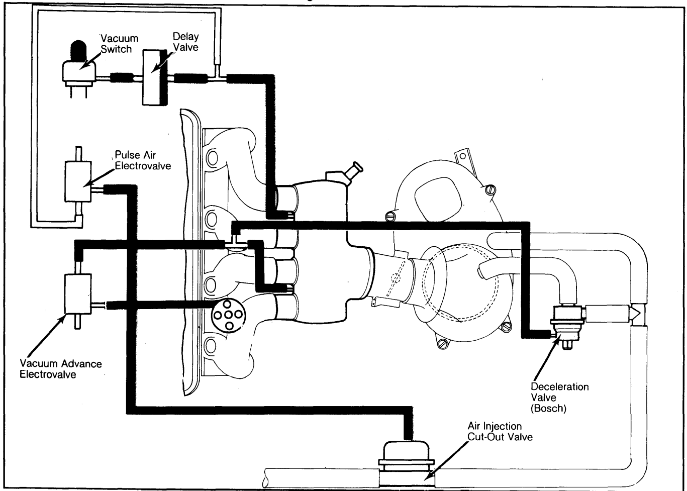
Fig. 1: Peugeot 505 Gasoline Model Vacuum Hose Diagram
