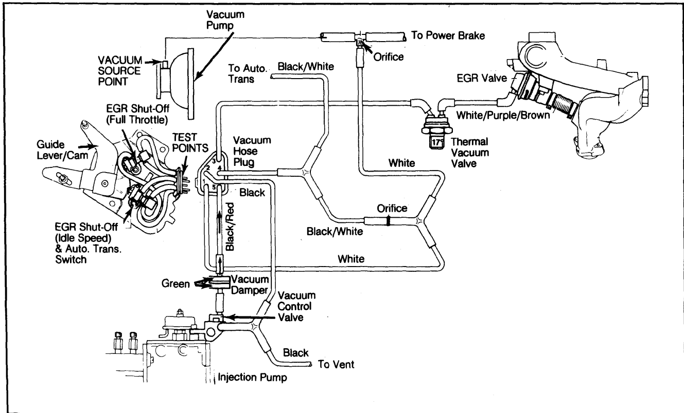
Fig. 2: 300 Series Non-Turbo Diesel Vacuum Hose Diagram
