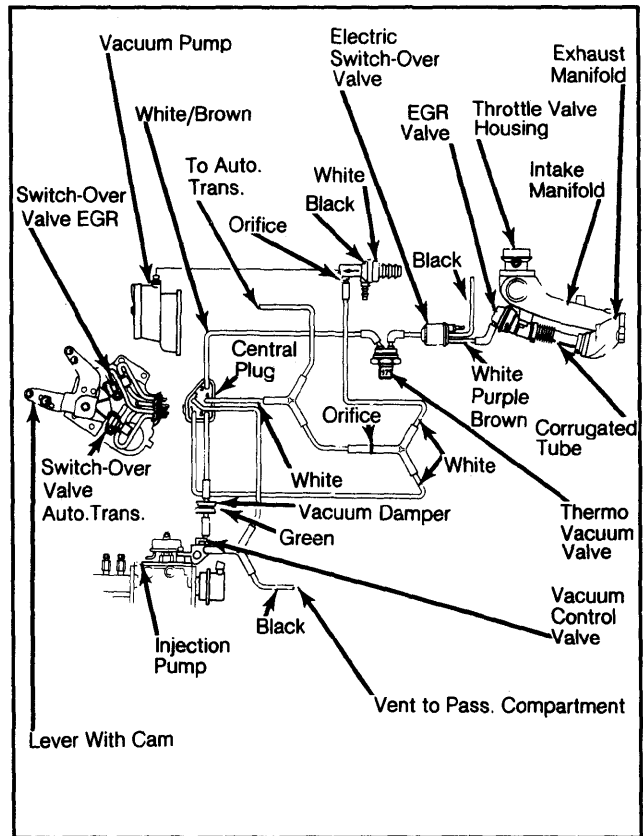
Fig. 3: 240D Auto. Trans. Diesel Vacuum Hose Diagram
