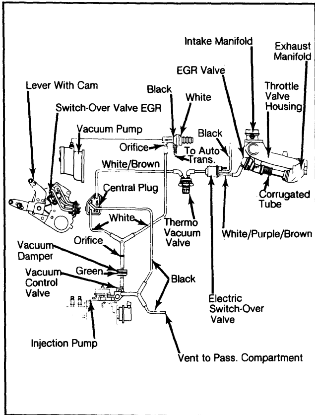
Fig. 1: 240D Man. Trans. Diesel Vacuum Hose Diagram
