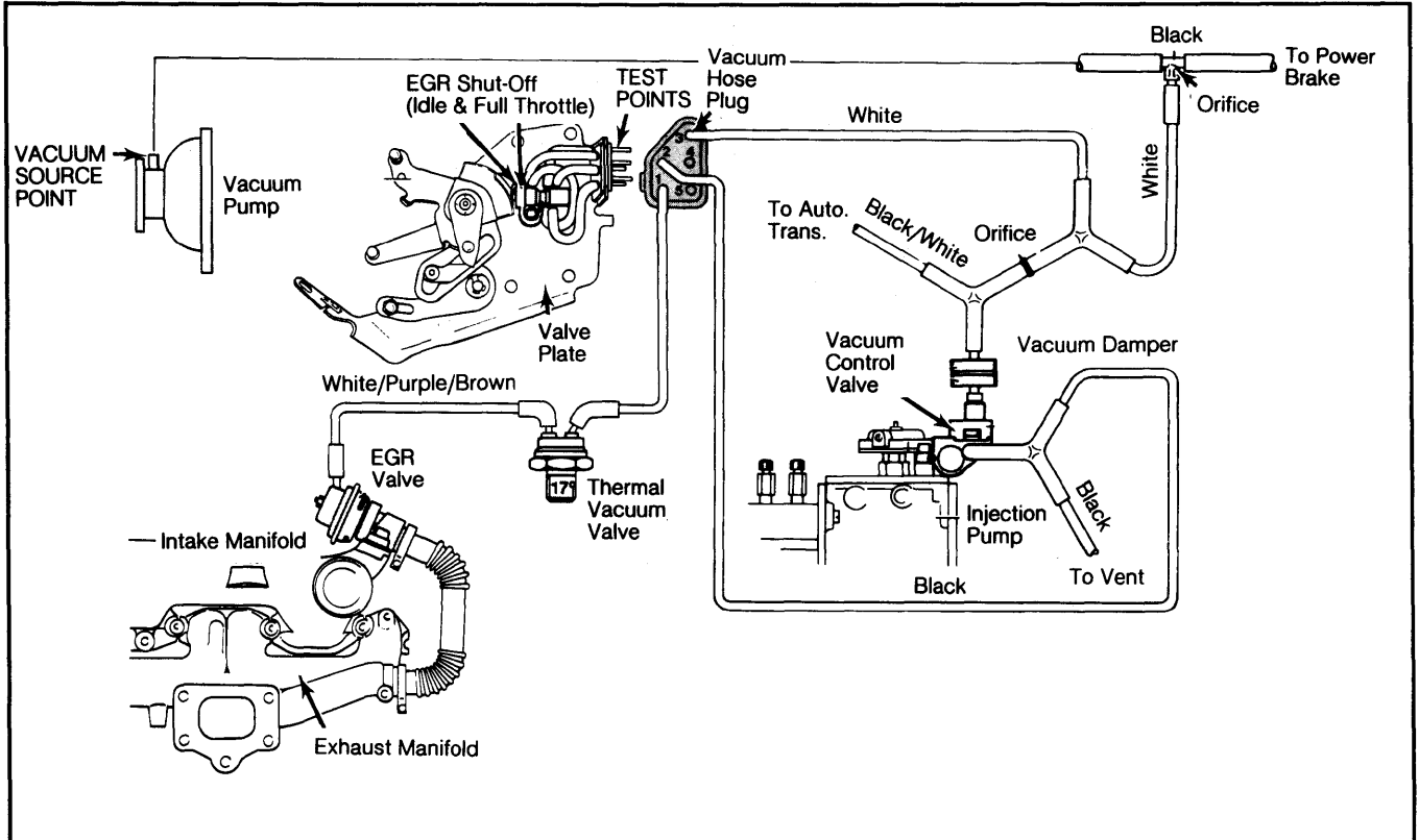
Fig. 5: 380 Series Vacuum Hose Diagram
