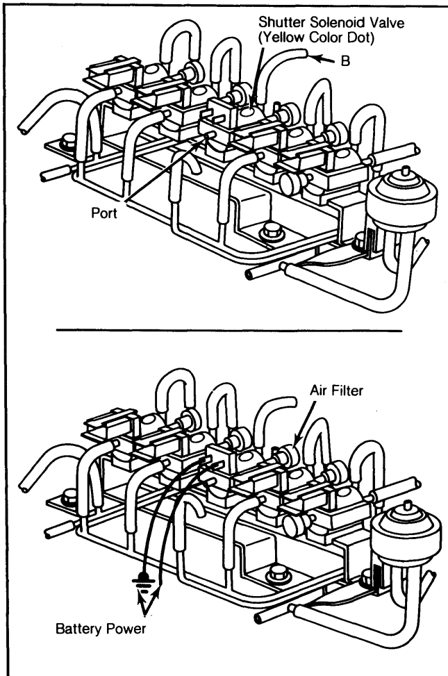
Fig. 3: Testing Shutter Solenoid Valve
