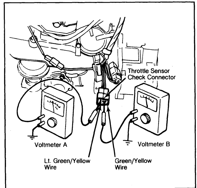
Fig. 2: Testing Throttle Sensor
