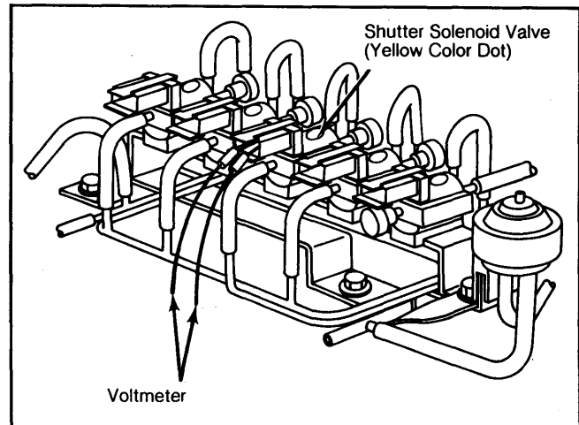
Fig. 4: Testing Shutter Solenoid Valve Signal
