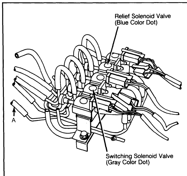
Fig. 1: Testing No. 1 Anti-Afterburn Valve
