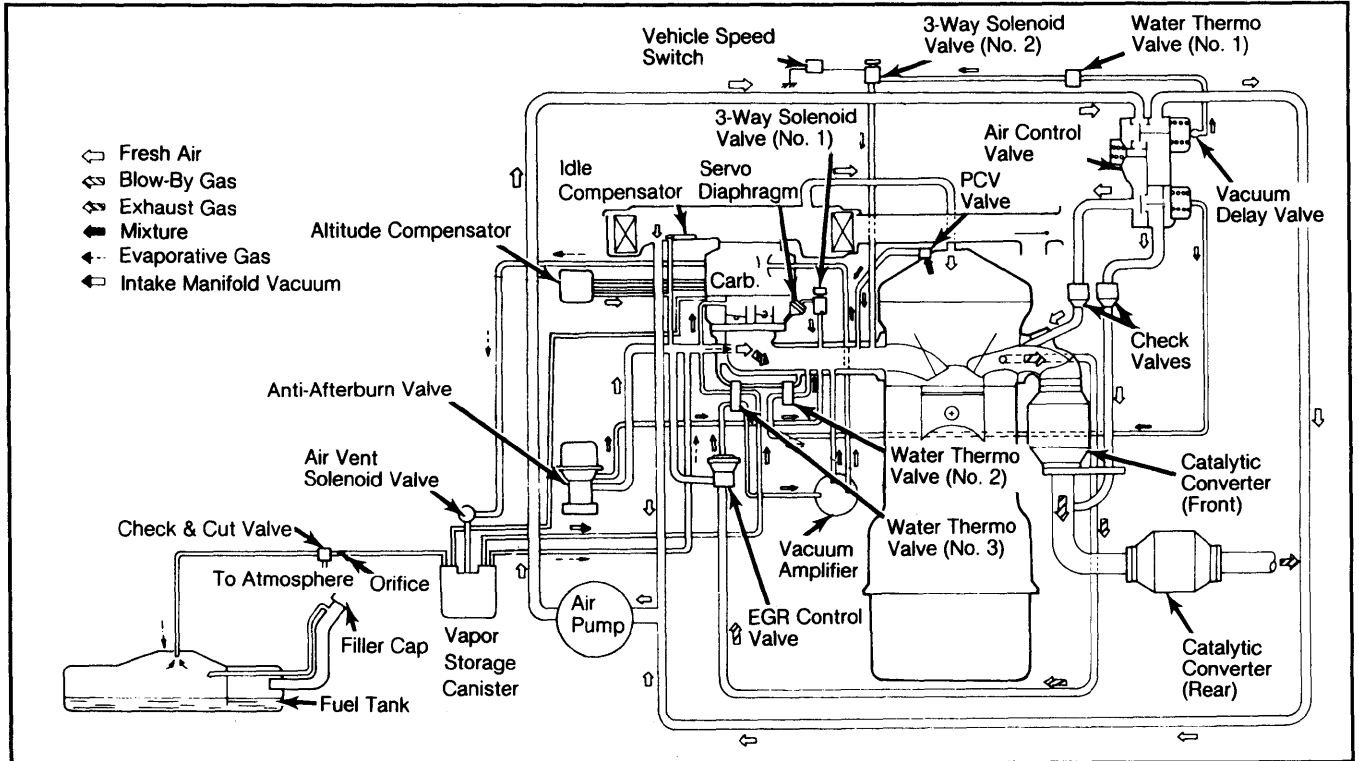
Fig. 3: Mazda GLC FWD Vacuum Diagram
