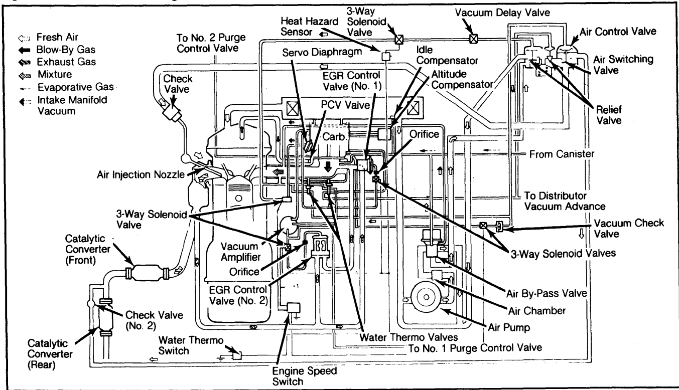
Fig. 5: Mazda 626 Vacuum Diagram
