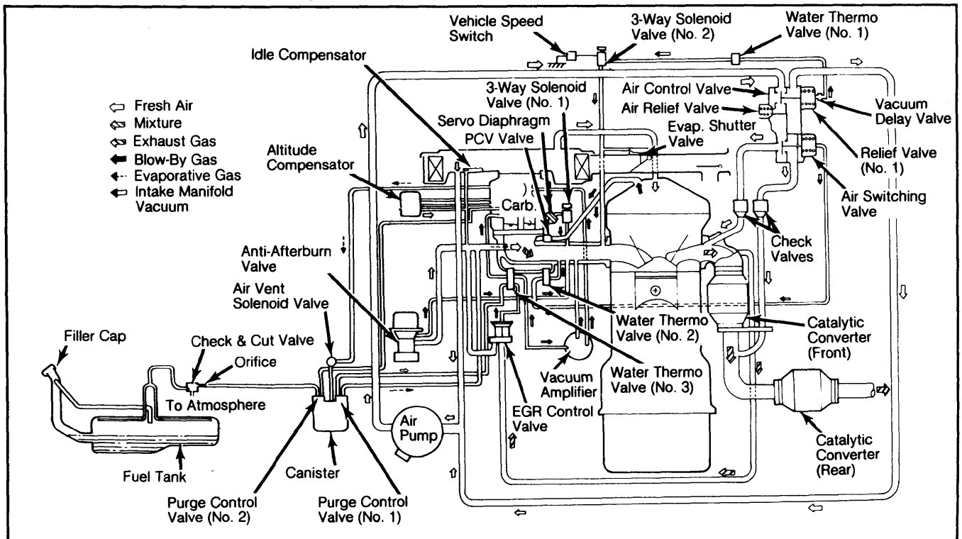
Fig. 4: Mazda GLC Wagon Vacuum Diagram
