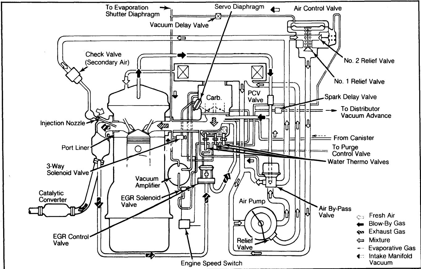
Fig. 2: Mazda B2000 Vacuum Diagram (Federal Models)
