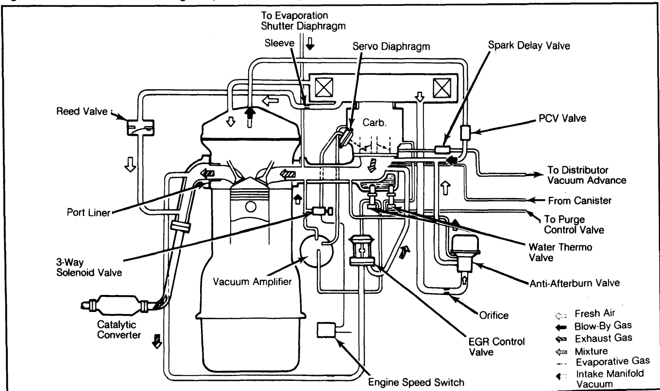
Fig. 2: Mazda B2000 Vacuum Diagram (Federal Models)
