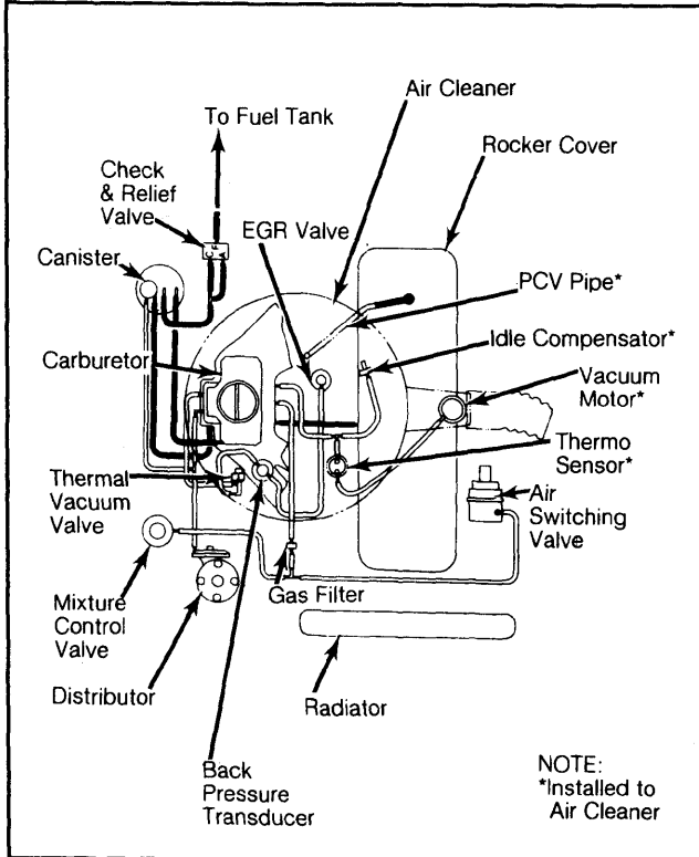
Fig. 2: Isuzu I-Mark Vacuum Diagram
