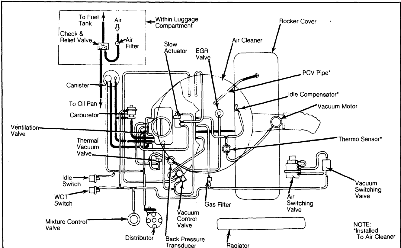
Fig. 2: Isuzu I-Mark Vacuum Diagram
