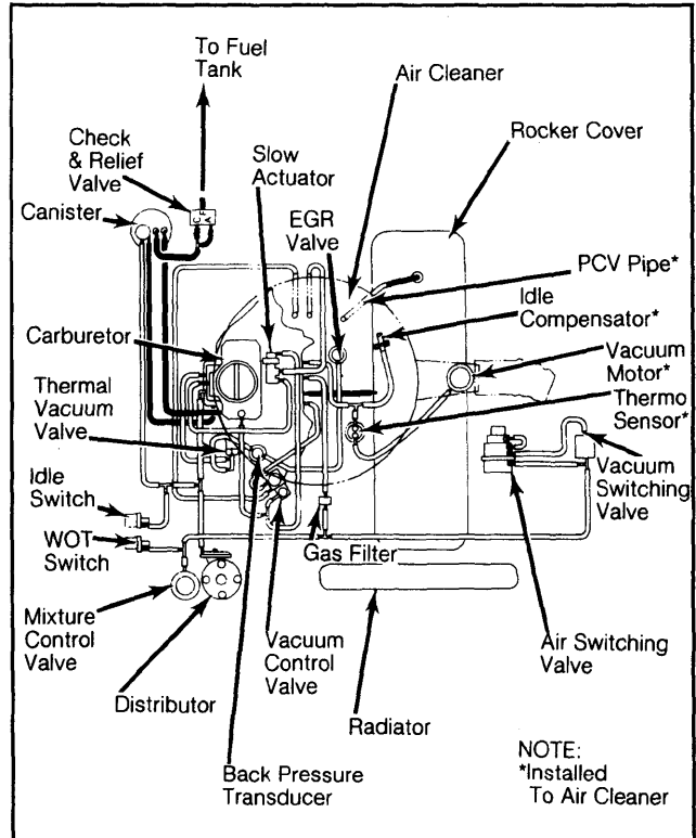
Fig. 3: California Isuzu P'UP and LUV Pickup Vacuum Diagram
