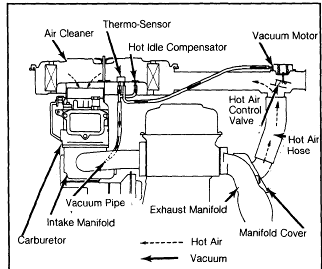
Fig. 1: Isuzu & LUV Thermostatic Air Cleaner Assembly
