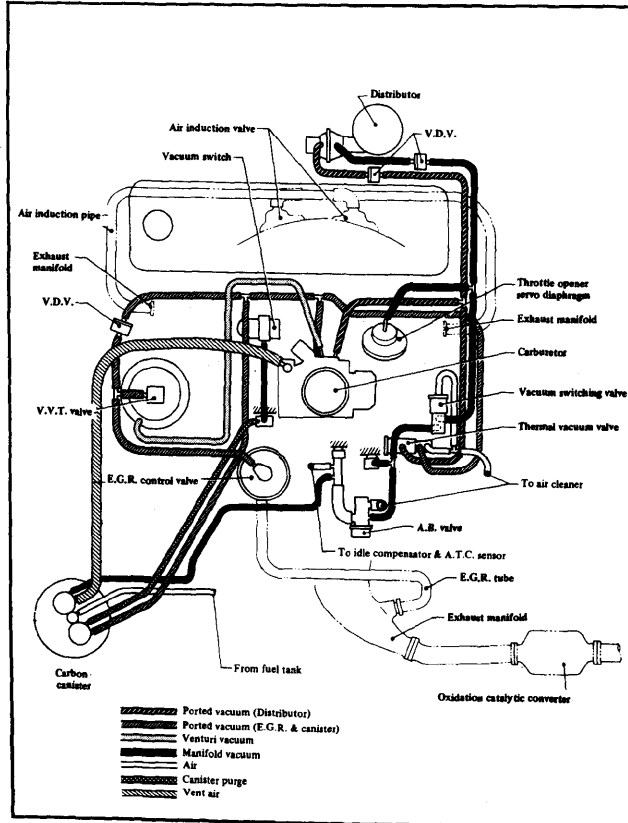
Fig. 14: Datsun 210 Vacuum Diagram (Federal)
