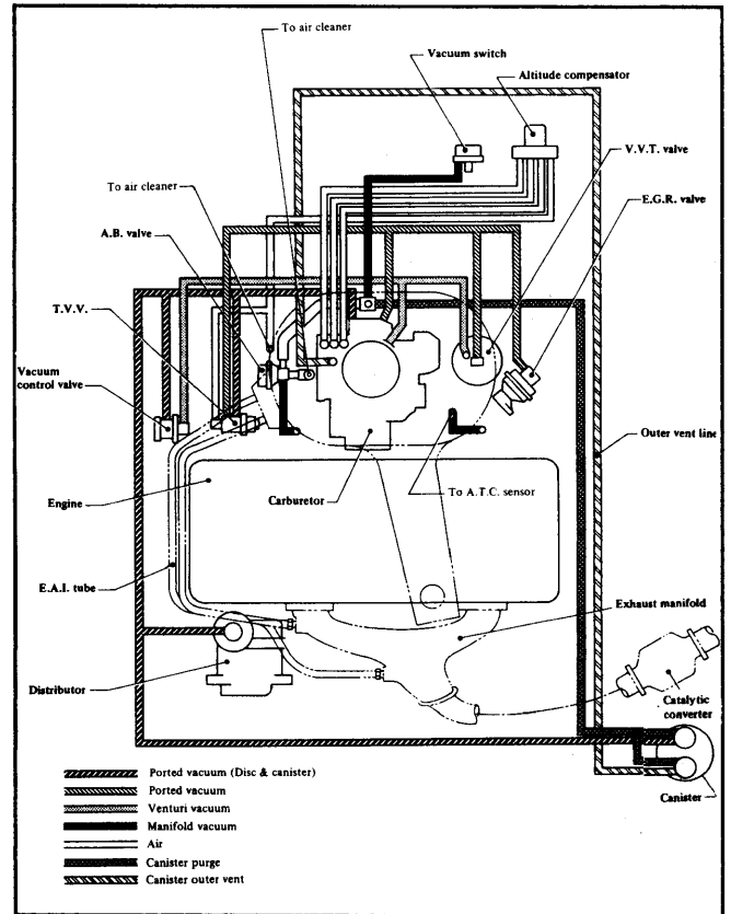
Fig. 11: Datsun Stanza Vacuum Diagram (High Altitude)
