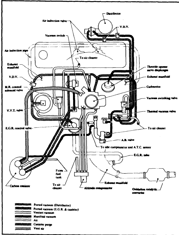
Fig. 13: Datsun 210 Vacuum Diagram (California)
