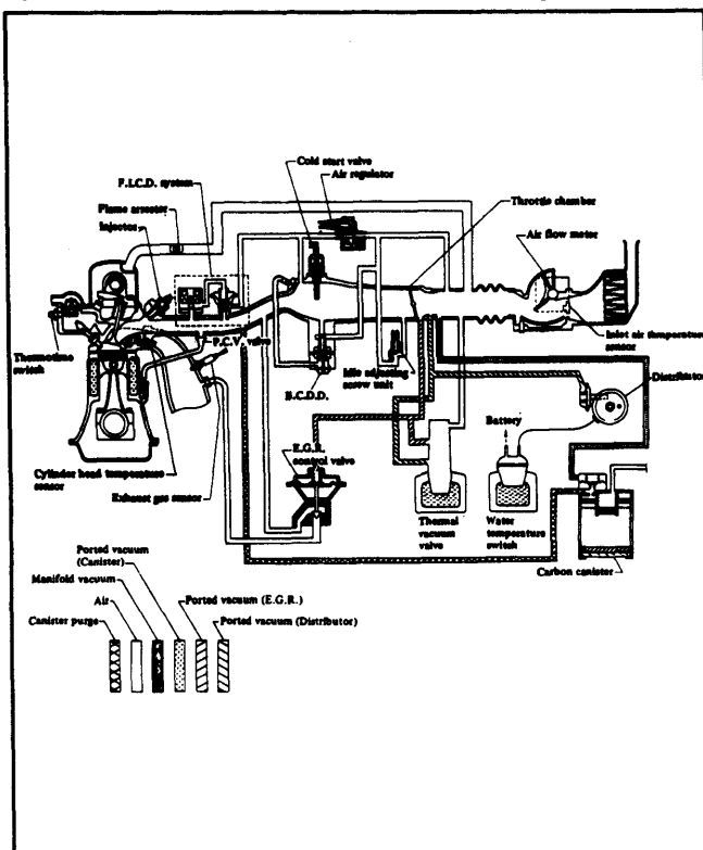
Fig. 2: Datsun Maxima Gasoline Vacuum Diagram
