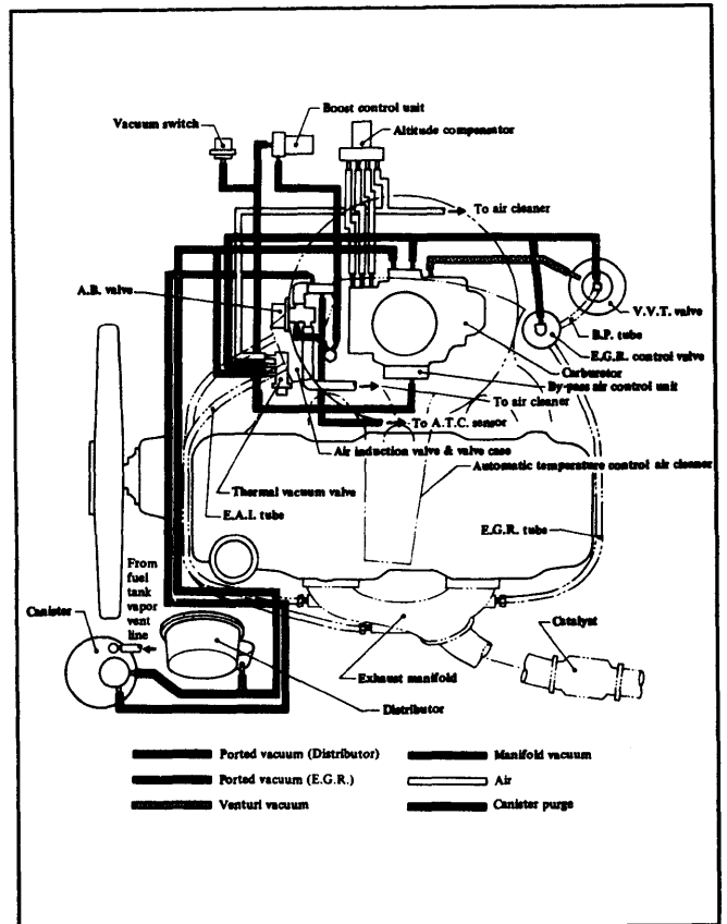
Fig. 3: Datsun Pickup Vacuum Diagram (California)
