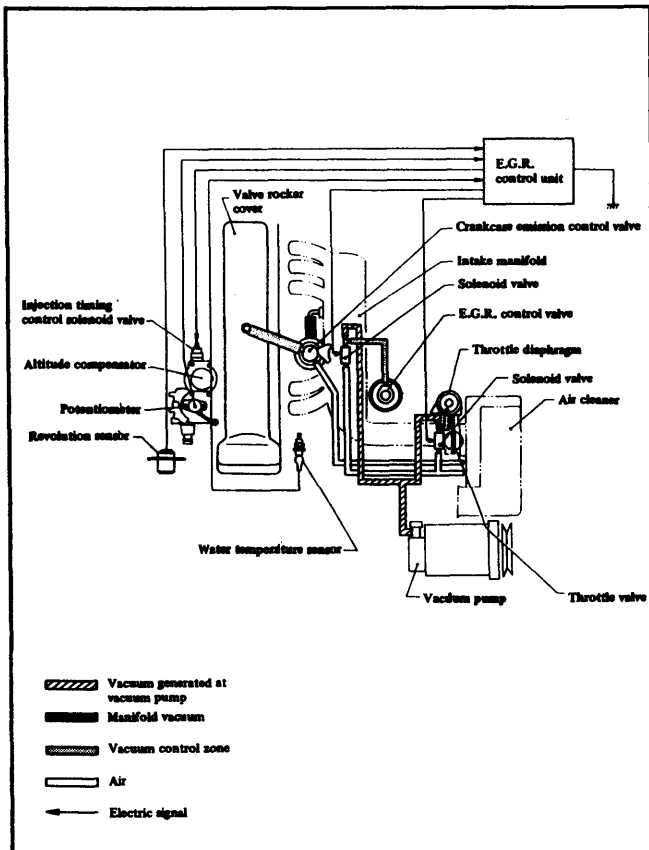
Fig. 1: Datsun Maxima Diesel Vacuum Diagram
