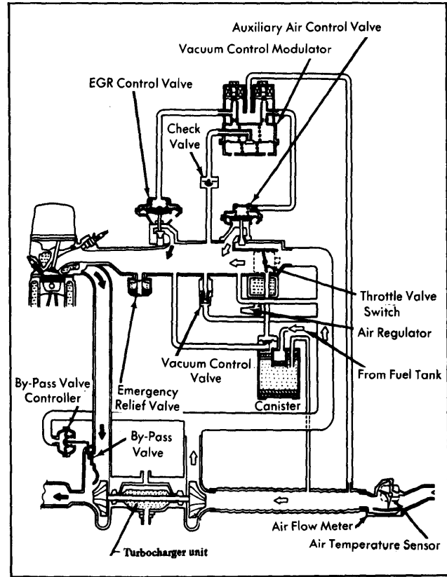
Fig. 16: Datsun 280ZX Turbo Vacuum Diagram
