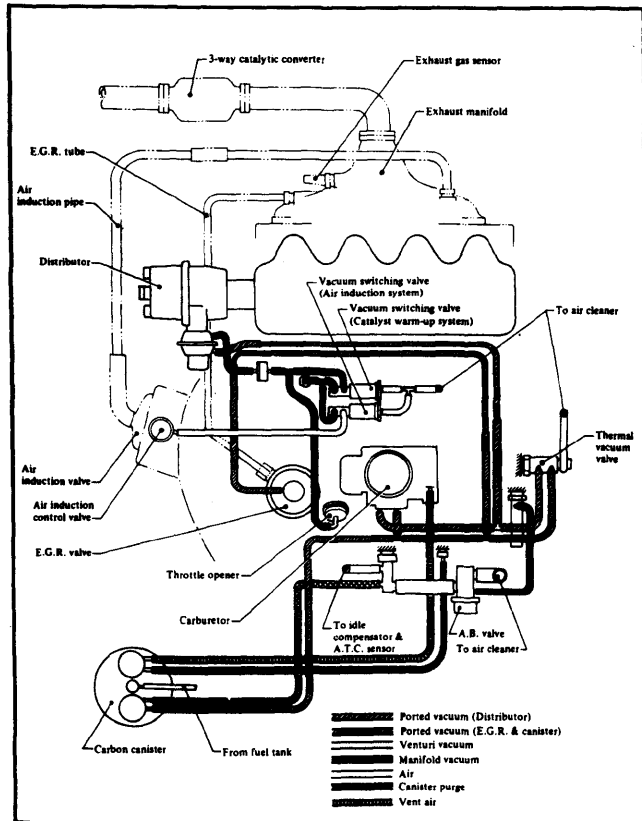
Fig. 6: Datsun Sentra M.P.G. Vacuum Diagram
