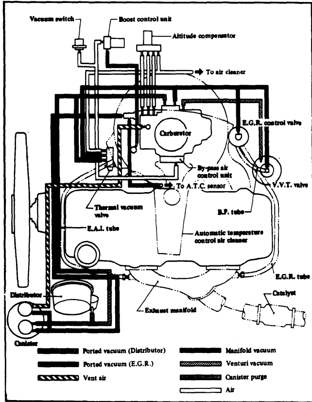
Fig. 5: Datsun Pickup Vacuum Diagram (High Altitude)
