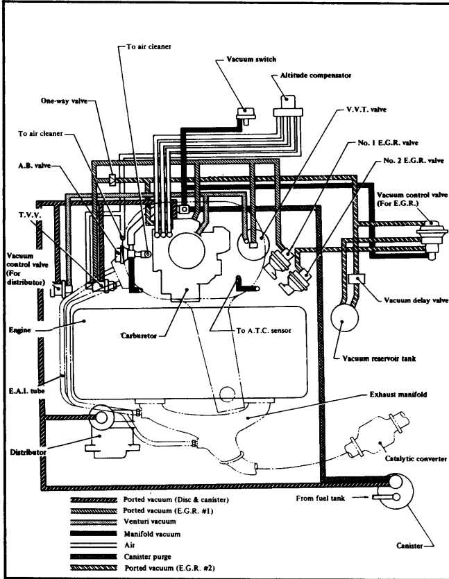
Fig. 9: Datsun Stanza Vacuum Diagram (California)
