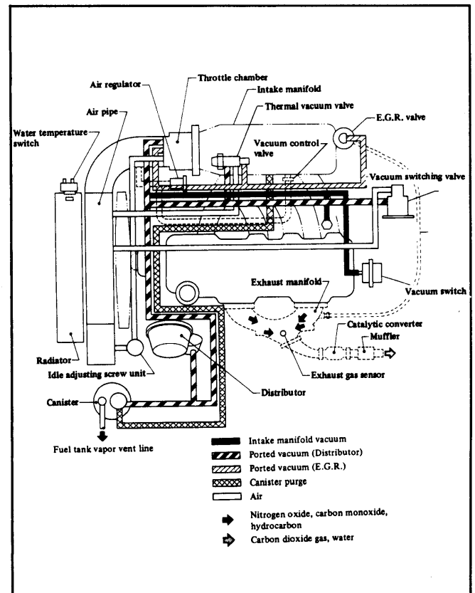
Fig. 12: Datsun 200SX Vacuum Diagram
