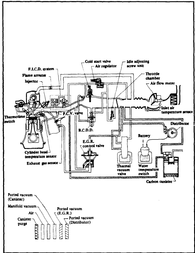
Fig. 15: Datsun 280ZX Vacuum Diagram
