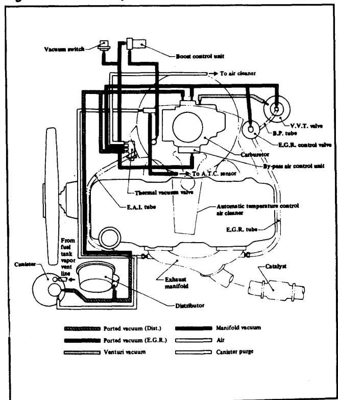
Fig. 4: Datsun Pickup Vacuum Diagram (Federal)
