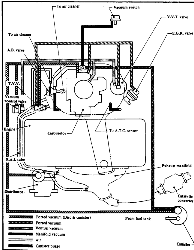
Fig. 10: Datsun Stanza Vacuum Diagram (Federal)
