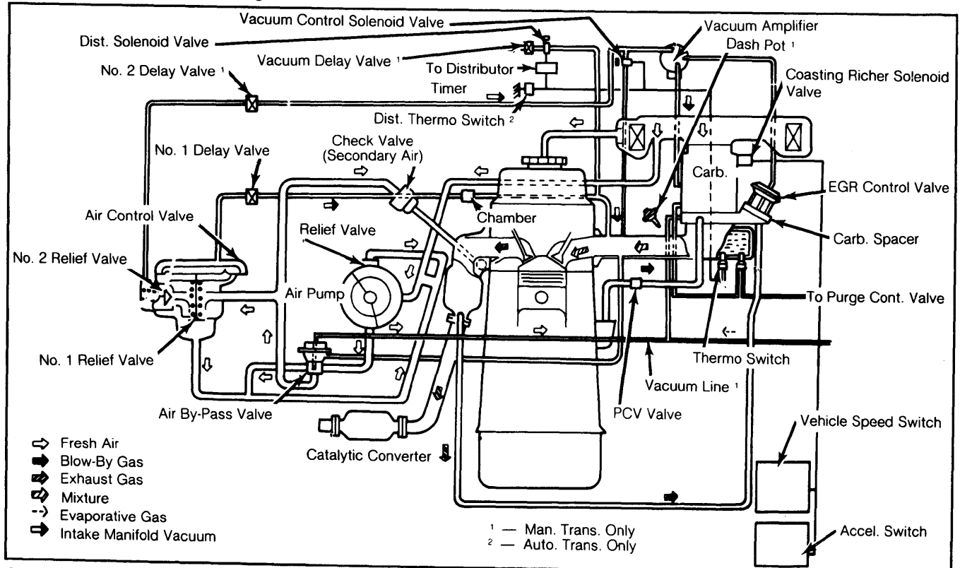
Fig. 4: 2.3L Engine Vacuum Diagram
