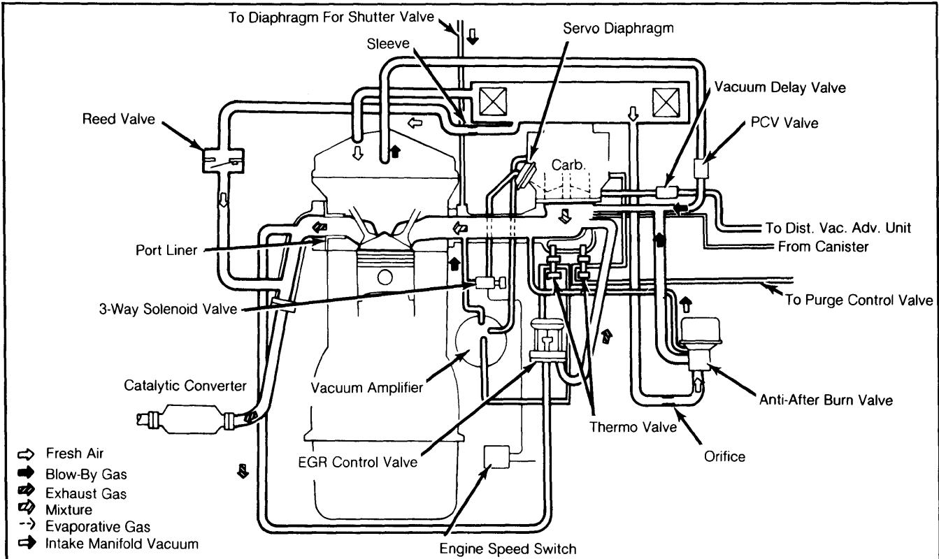
Fig. 1: 2.0L Engine Vacuum Diagram
