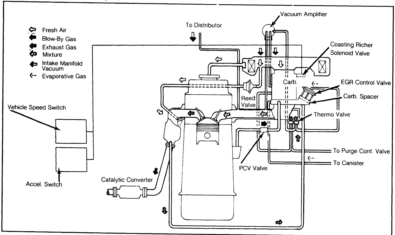
Fig. 3: 2.3L Engine Vacuum Diagram
