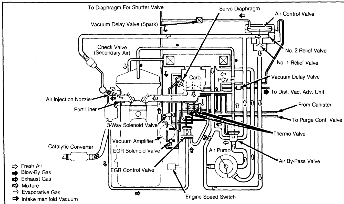
Fig. 2: 2.0L Engine Vacuum Diagram
