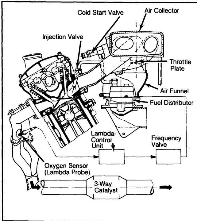
Fig. 1: BMW 320i Exhaust Emission Control System Vacuum Diagram
