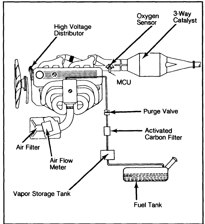
Fig. 3: BMW 528e Exhaust Emission Control System Vacuum Diagram
