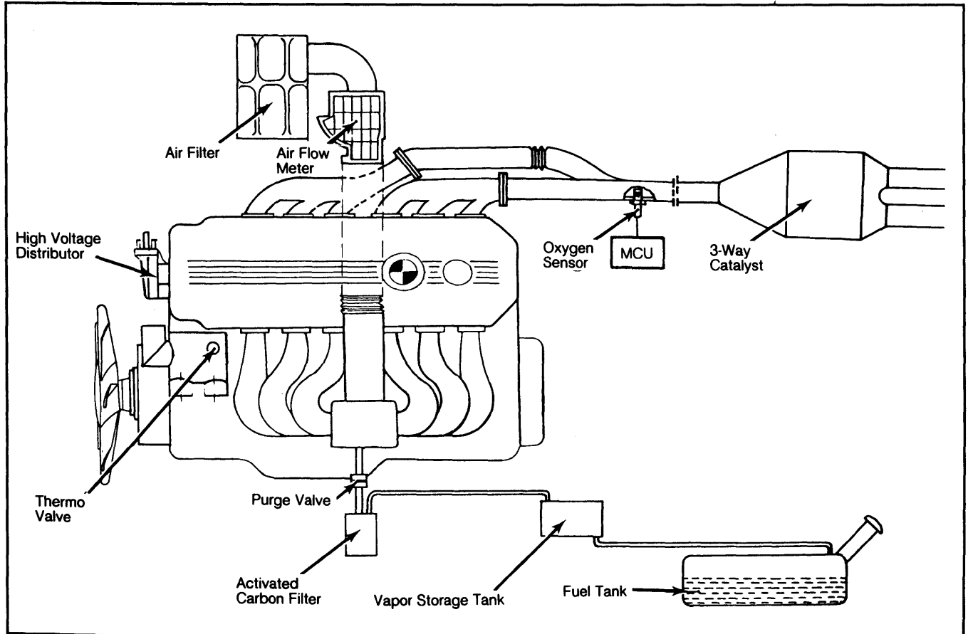
Fig. 2: BMW 633CSi & 733i Exhaust Emission Control System Vacuum Diagram
