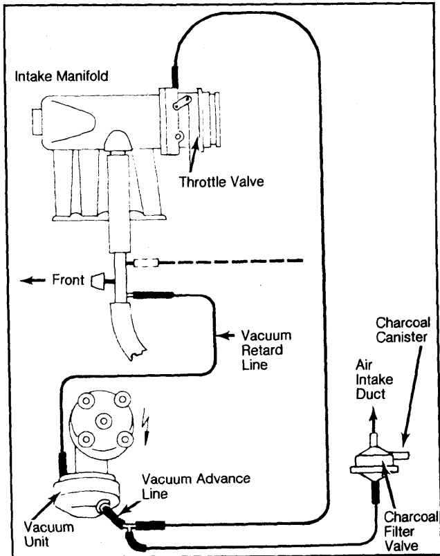
Fig. 1: Audi 4000 Vacuum Diagram (4-Cylinder)
