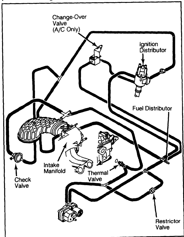
Fig. 4: Audi 5000 Vacuum Diagram (Non-Turbocharged Models)
