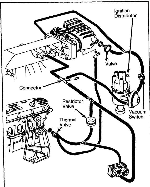
Fig. 2: Audi 4000 Vacuum Diagram (5-Cylinder Models)
