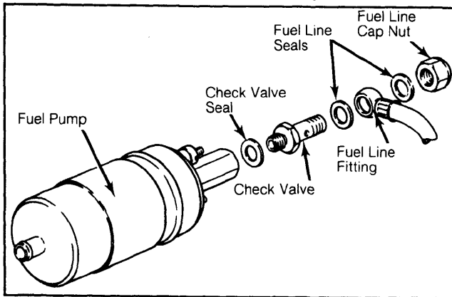
Fig. 1: View of Bosch Electric Fuel Pump
