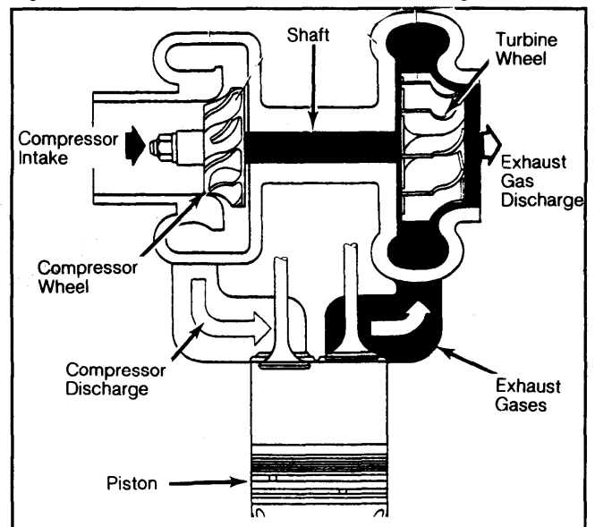
Fig. 3: Airflow Pattern with Garrett Turbocharger
