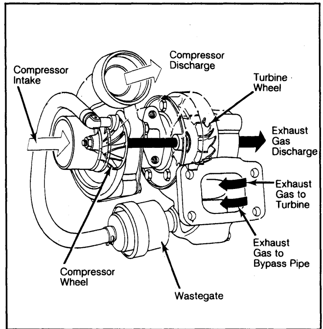
Fig. 2: Cutaway View of Garrett Turbocharger
