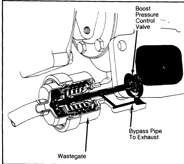
Fig. 4: Cutaway View of Wastegate Valve
