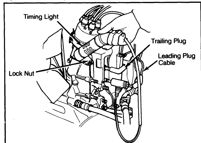
Fig. 2: Connecting Timing Light
