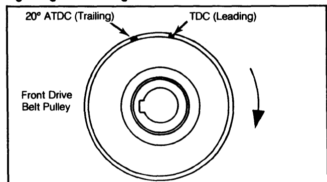
Fig. 3: Ignition Timing Mark Location
