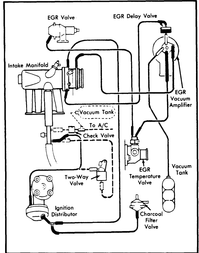
Fig. 2 Volkswagen Vacuum Diagram (Rabbit Pickup)
