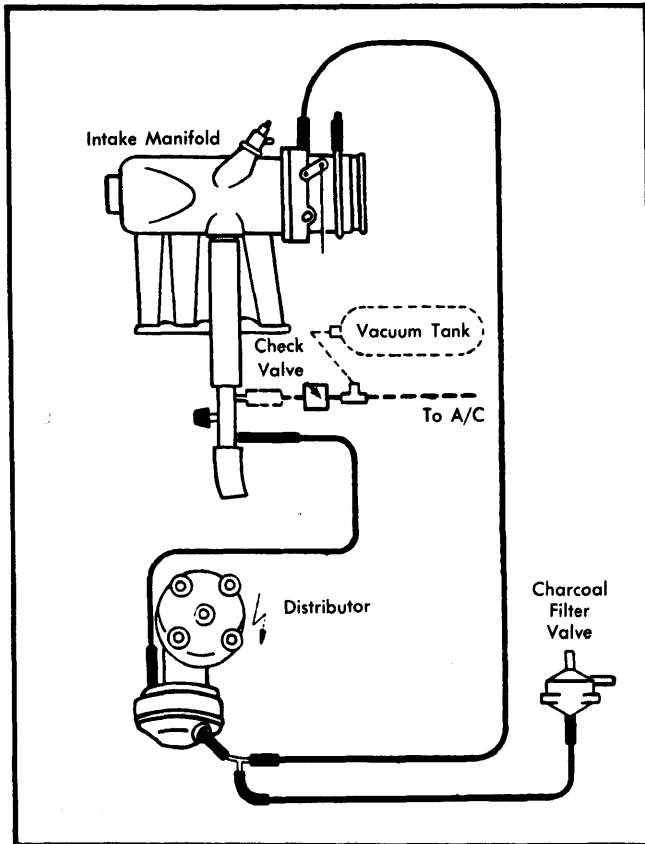
Fig. 1 Volkswagen Vacuum Diagram (Dasher, Jetta, Rabbit & Scirocco)
