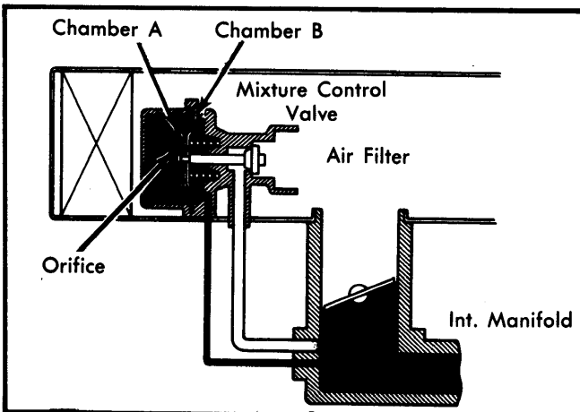
Fig. 1 Typical Mixture Control System
