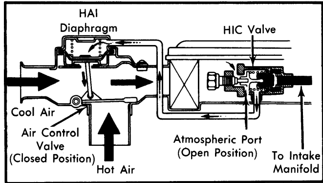
Fig. 1 HIC Valve Type Thermostatic Air Cleaner (Thermo Valve Type Similar)
