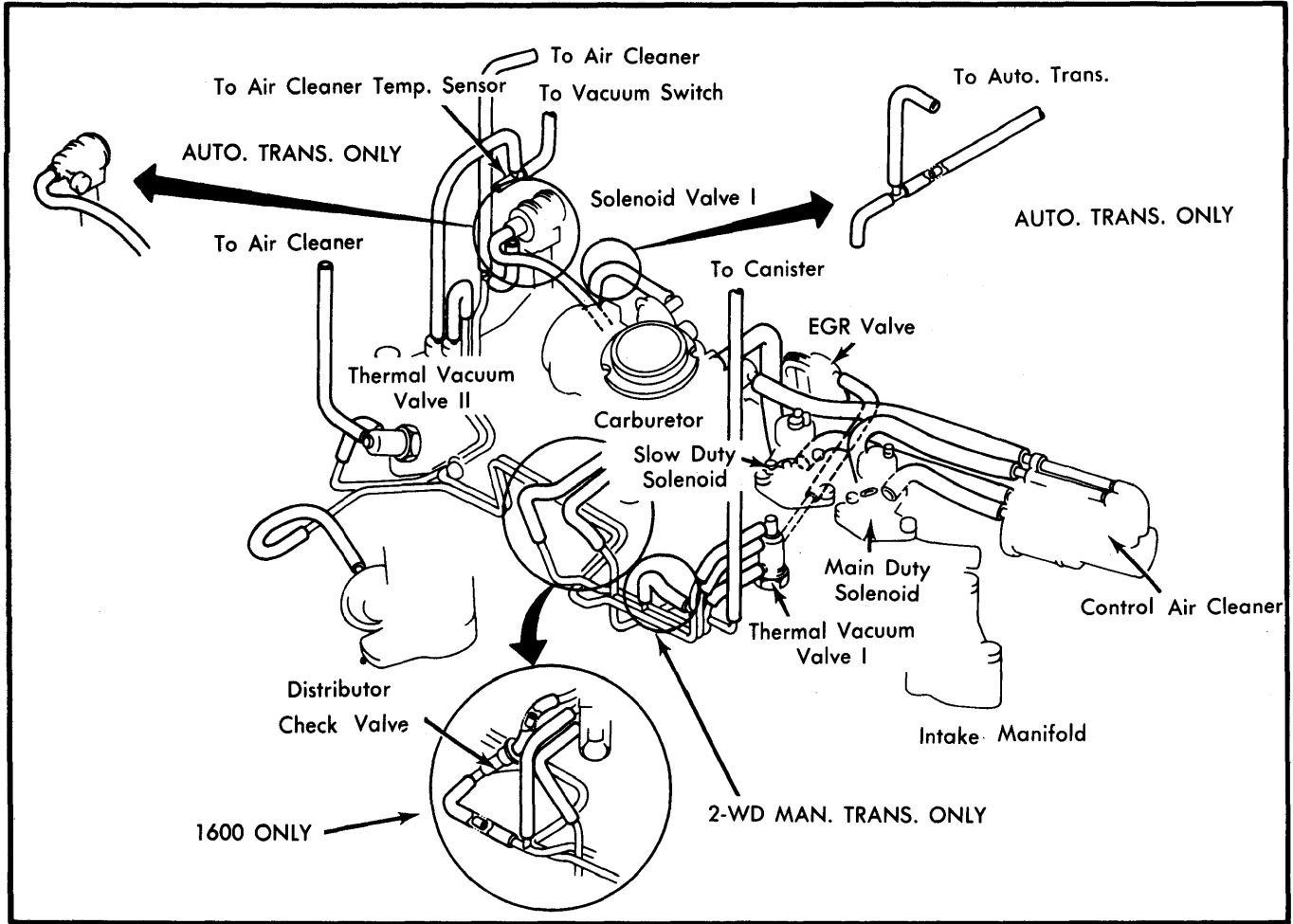
Fig. 1 Subaru Vacuum Diagram (All Models)
