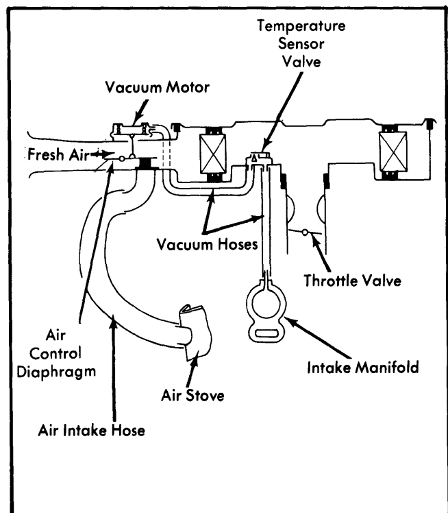
Fig. 1 Cutaway View of Thermostatic Air Cleaner
