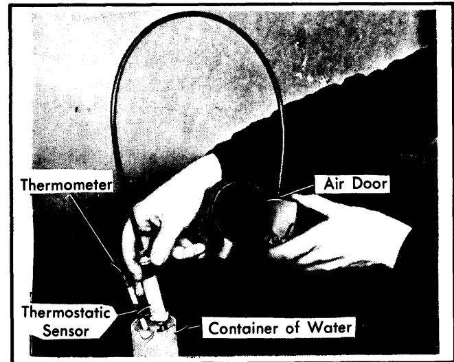
Fig. 1 Checking Thermostatic Air Cleaner Sensor (Non-Turbo Models)
