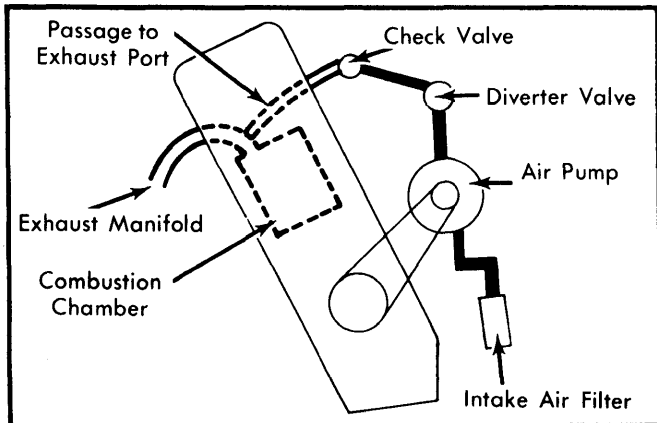
Fig. 1 Schematic of Porsche Air Injection System (924 Model Application Shown)
