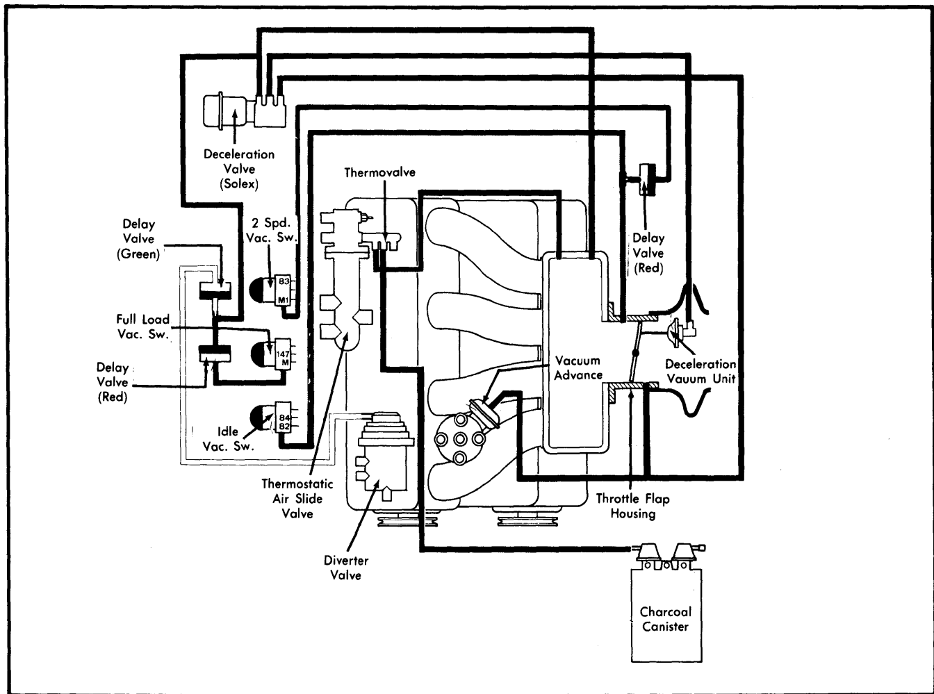
Fig. 1 505 Vacuum Hose Diagram
