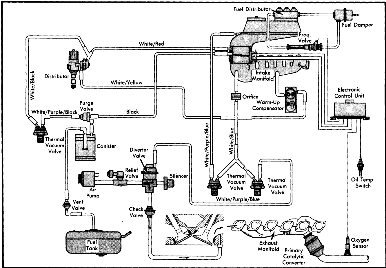
Fig. 1 280 Series Vacuum Hose Diagram
