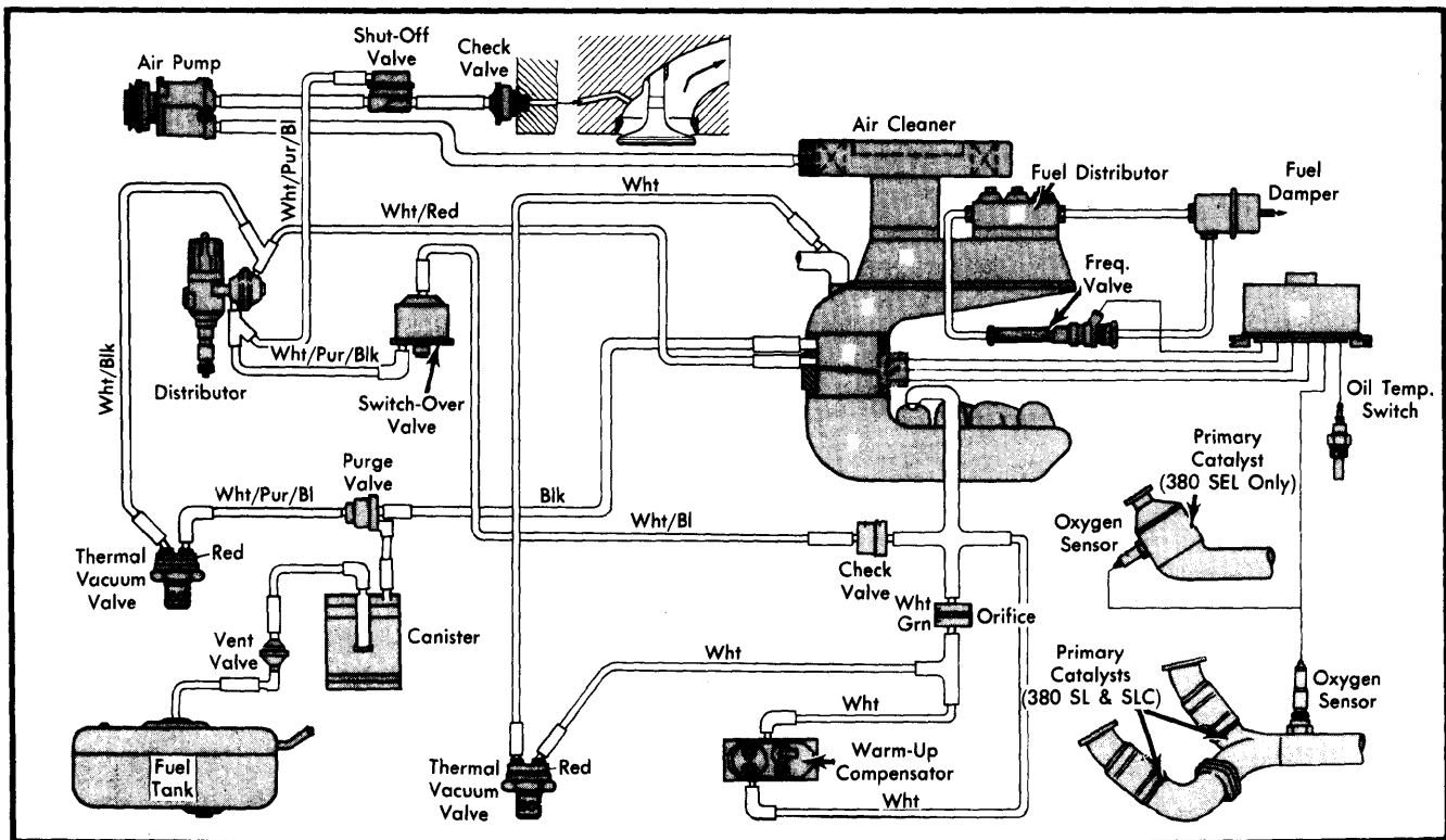
Fig. 2 380 Series Vacuum Hose Diagram
