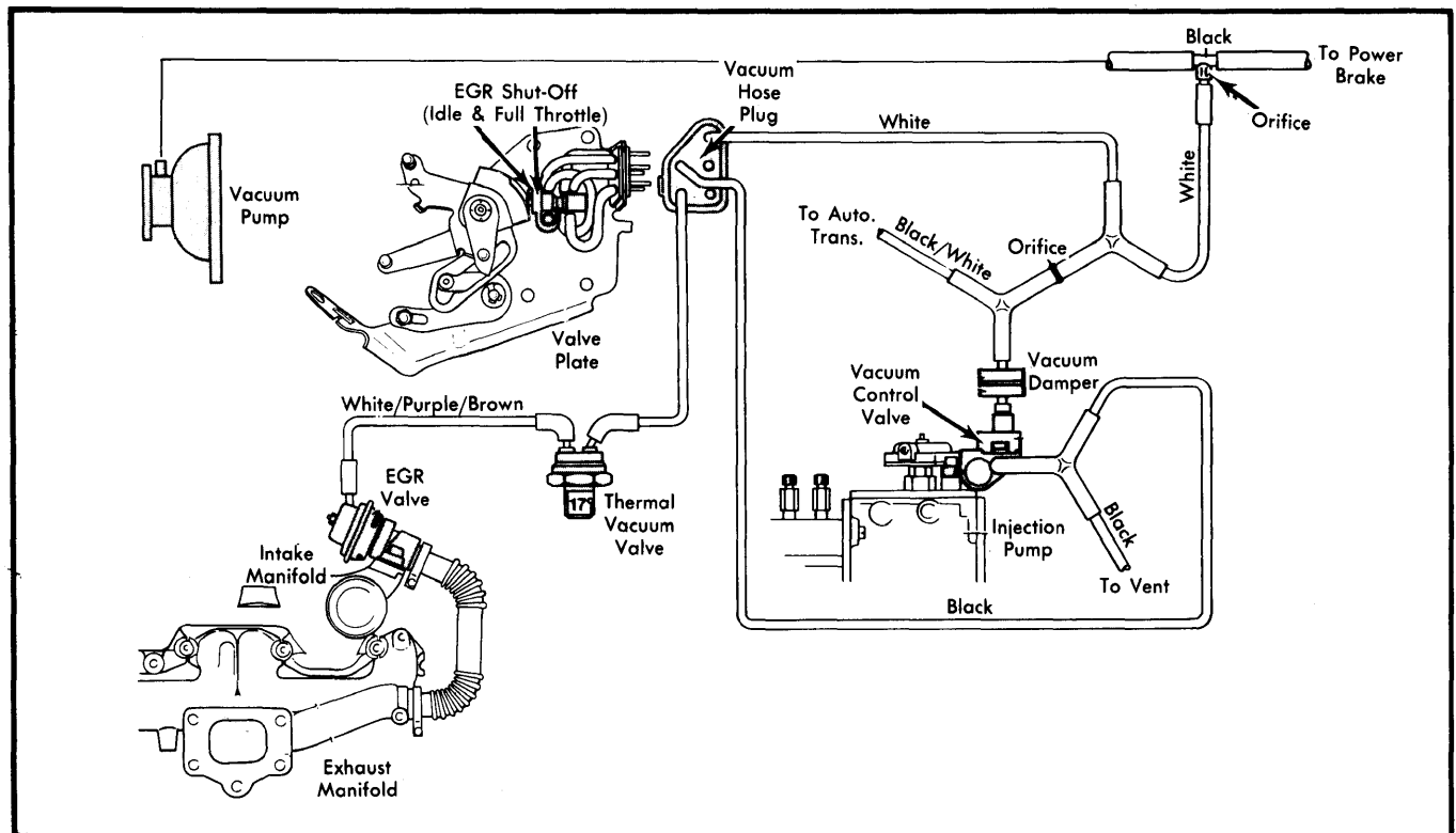
Fig. 4 300 Series Vacuum Hose Diagram (Turbo Diesel)
