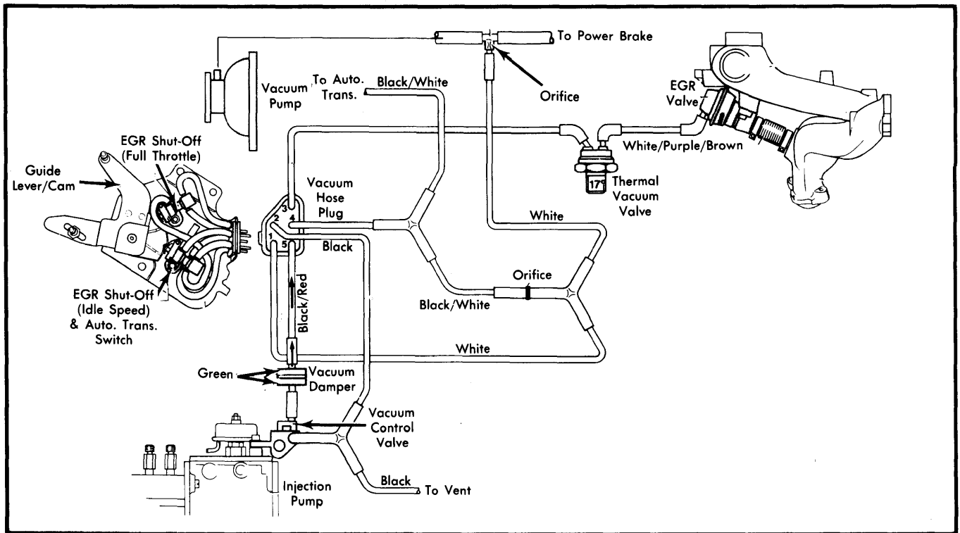
Fig. 3 300 Series Vacuum Hose Diagram (Except Turbo)
