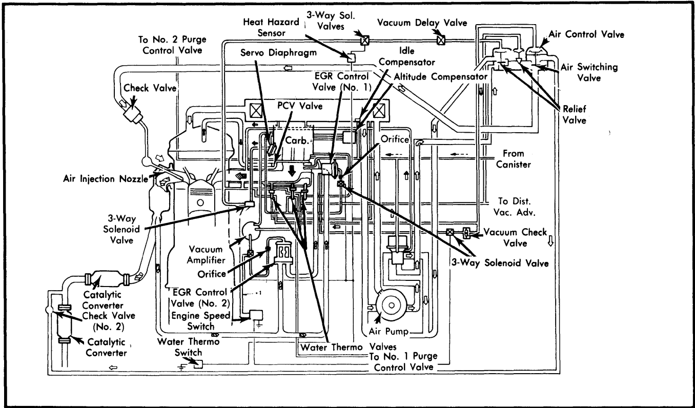
Fig. 3 Mazda 626 Vacuum Hose Routing
