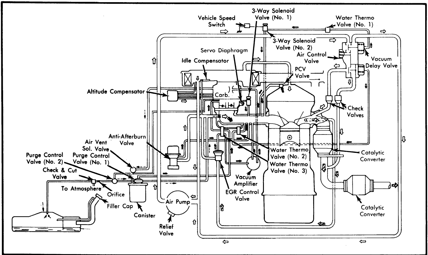
Fig. 1 Mazda GLC Vacuum Hose Routing
