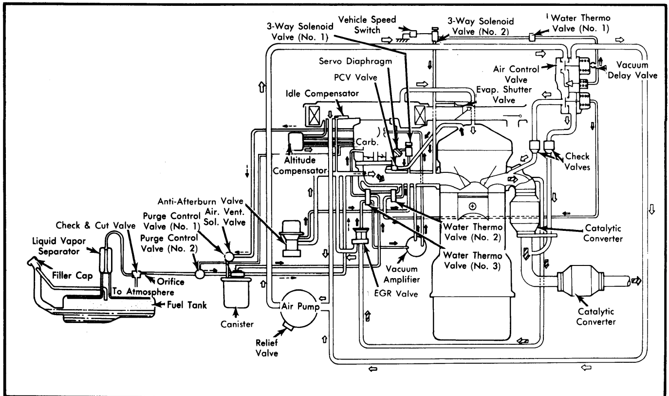
Fig. 2 Mazda GLC Wagon Vacuum Hose Routing
