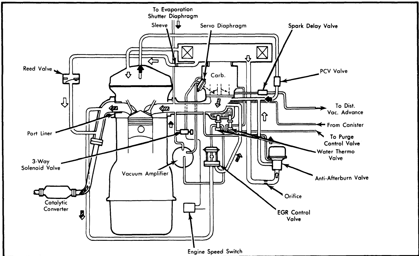
Fig. 3 Mazda 626 Vacuum Hose Routing
