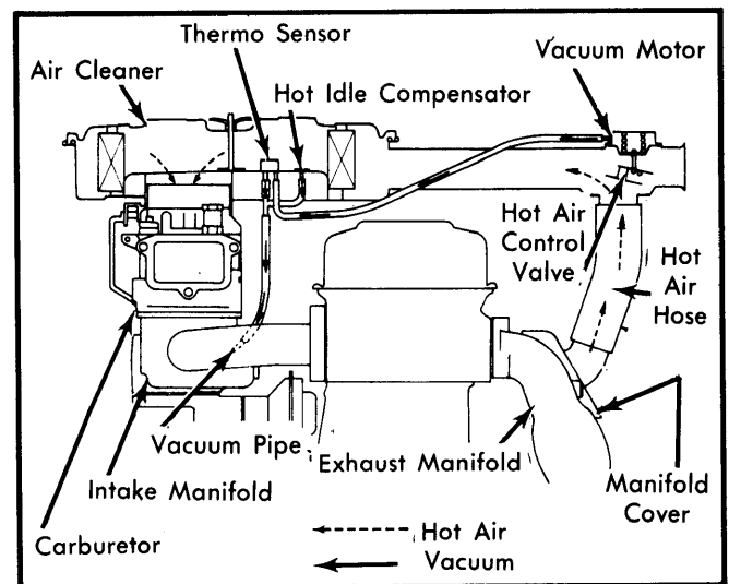
Fig. 1 Thermostatically Controlled Air Cleaner System
