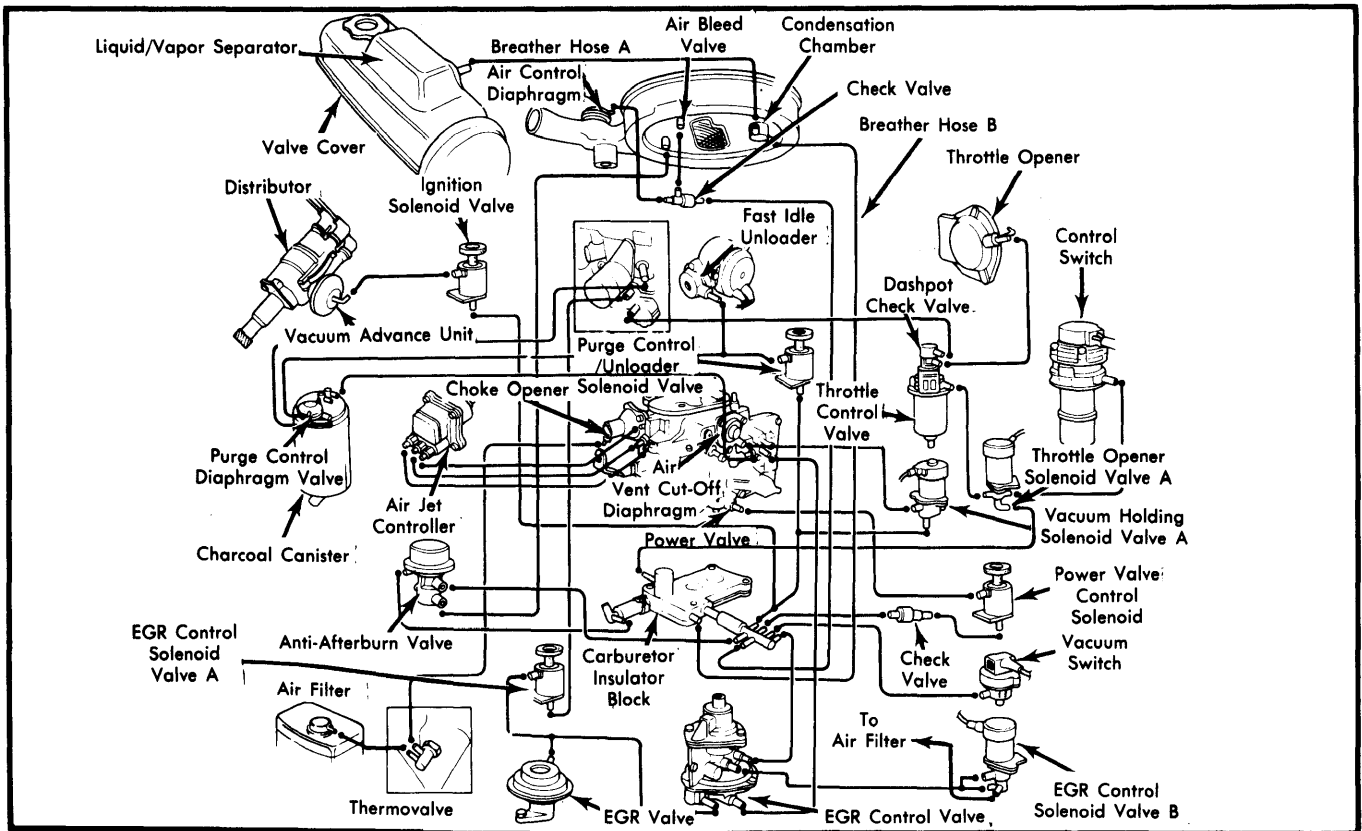
Fig. 2 Civic 1300 Calif. Models
