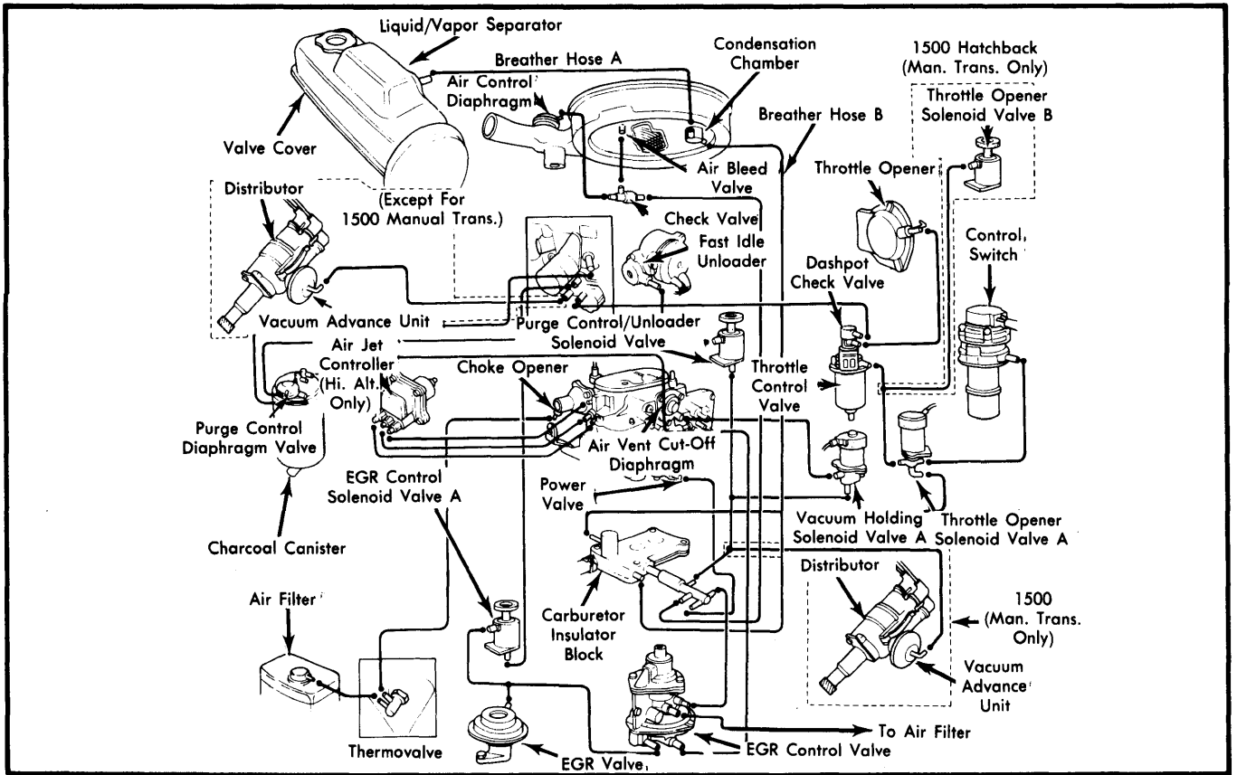
Fig. 1 Civic 1300 & 1500 Federal Models
