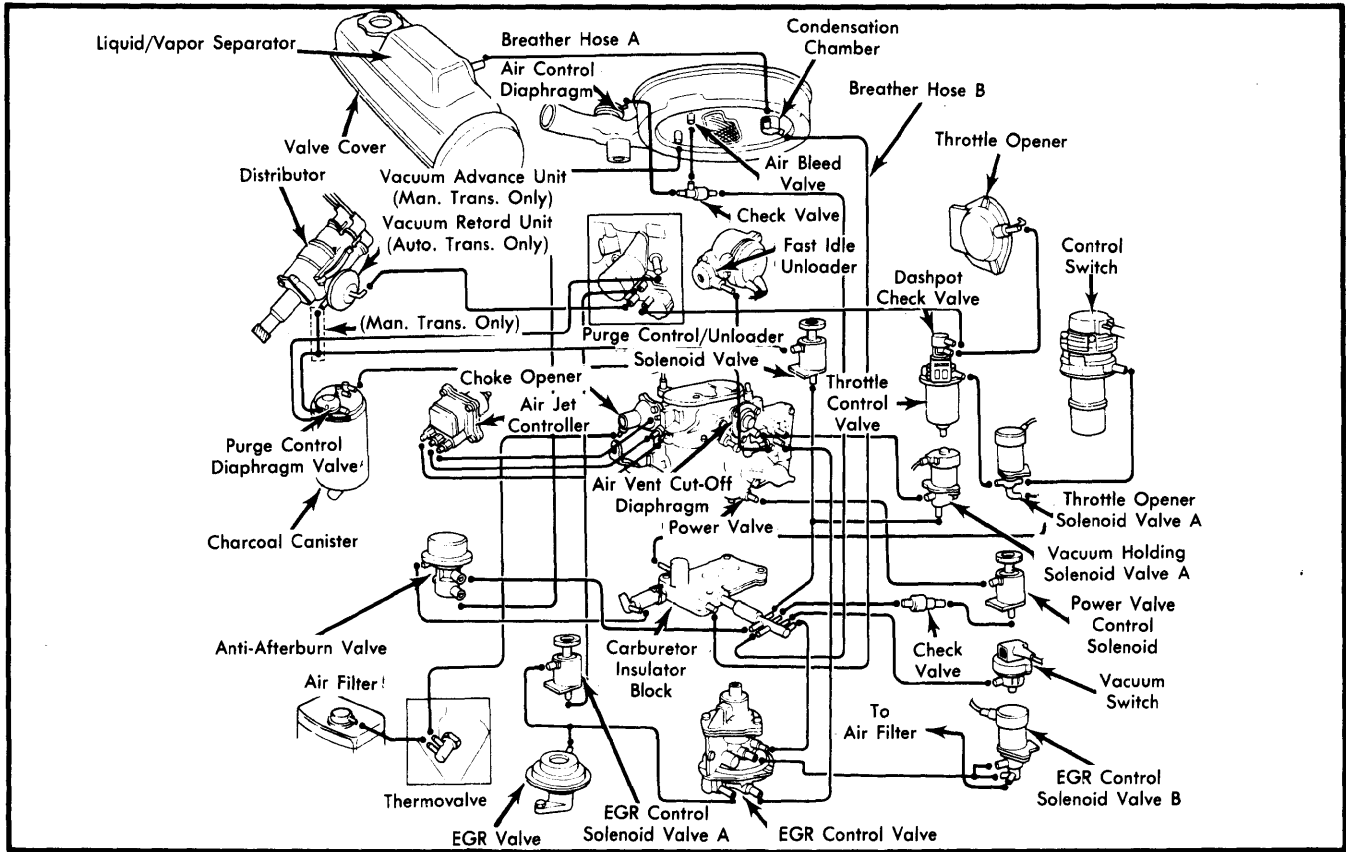
Fig. 3 Civic 1500 Calif. Models
