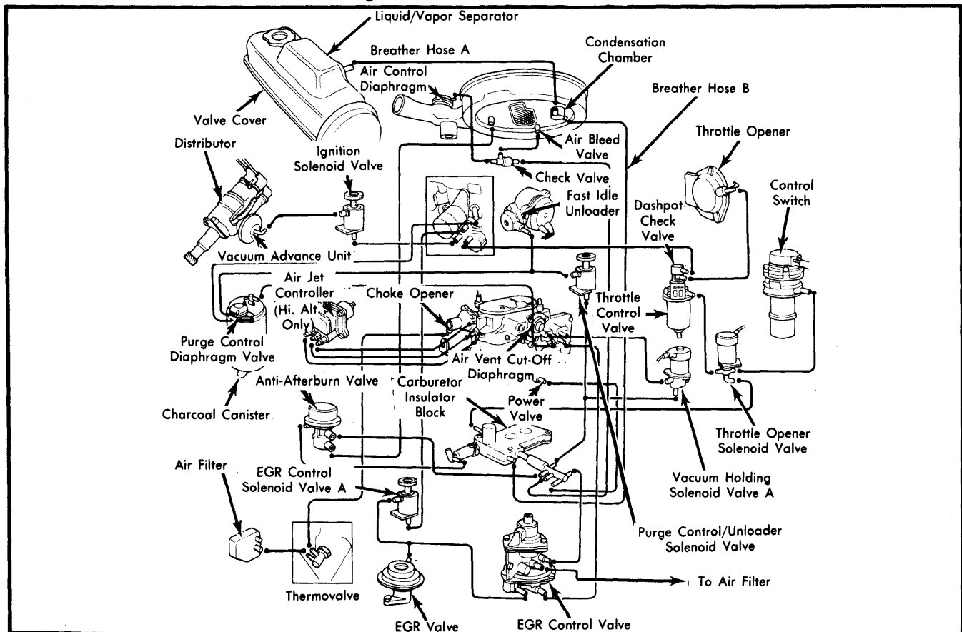
Fig. 4 Accord & Prelude Federal Man. Trans.
