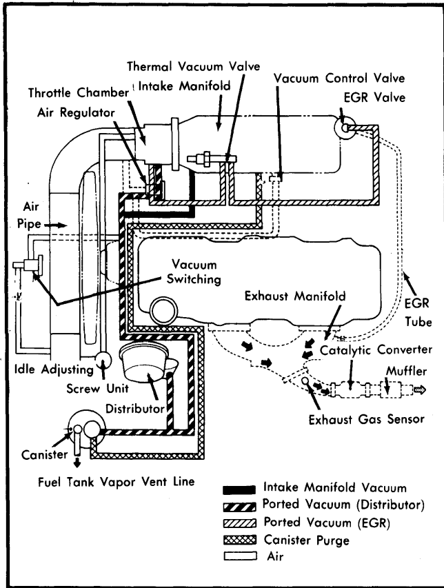
Fig. 1 Datsun 200SX Vacuum Diagram
