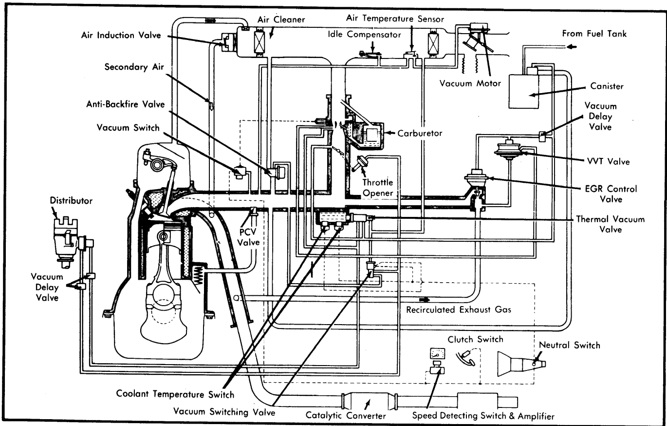
Fig. 8 Datsun 310 Vacuum Diagram (Federal)
