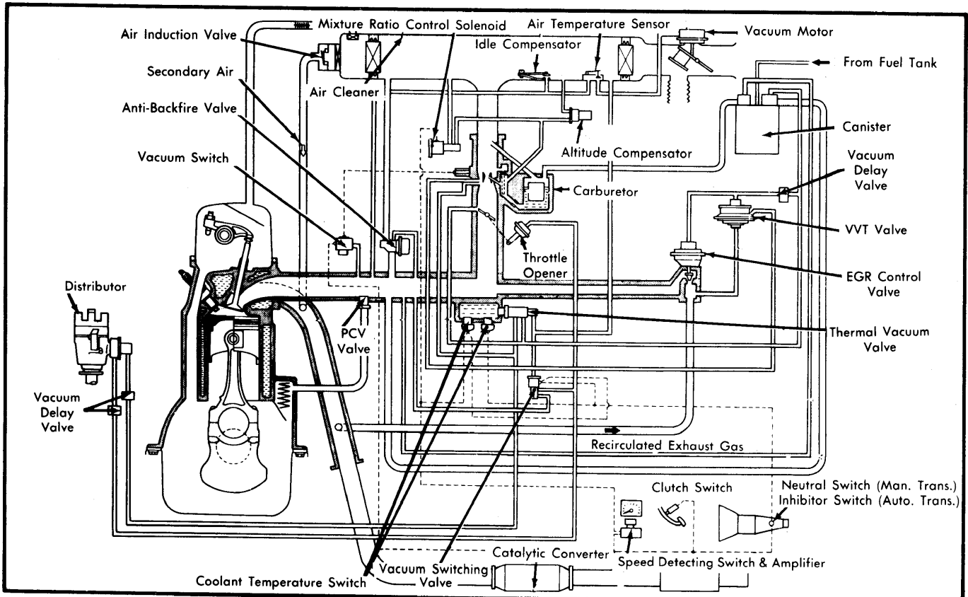
Fig. 9 Datsun 210 & 310 Vacuum Diagram (Calif.)
