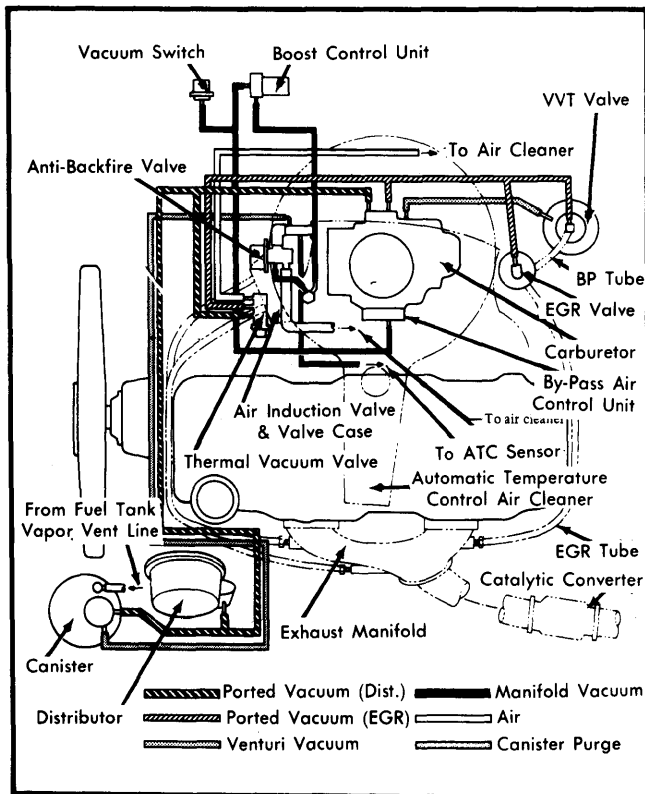
Fig. 2 Datsun 510 Vacuum Diagram (Federal)
