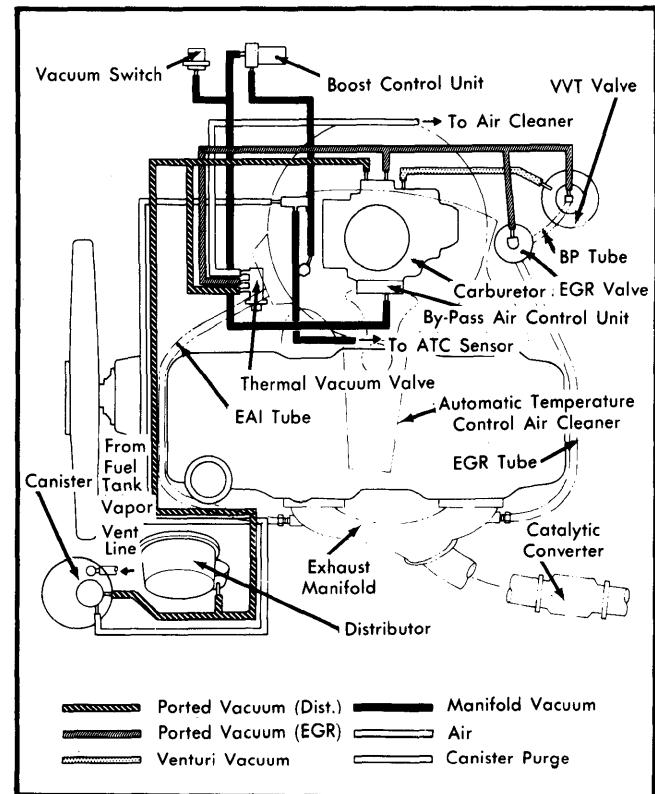
Fig. 4 Datsun Pickup Vacuum Diagram (Federal)
