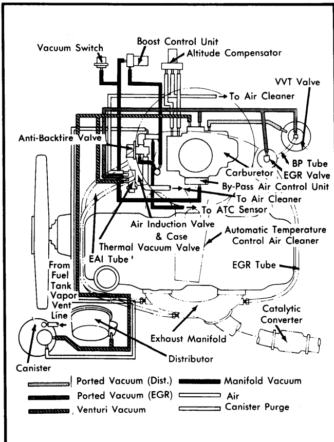
Fig. 5 Datsun Pickup Vacuum Diagram (Calif.)
