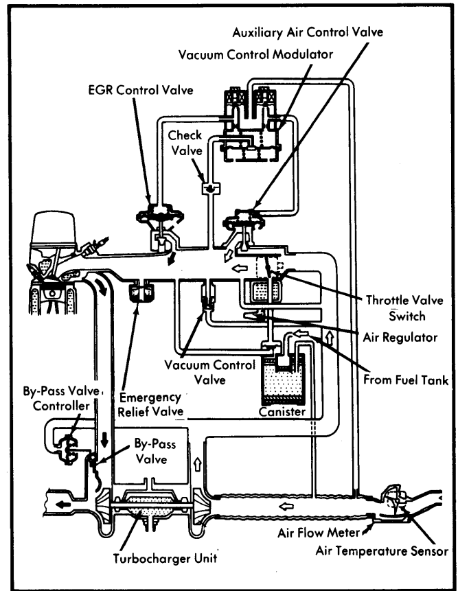
Fig. 6 Datsun 280ZX Turbo Vacuum Diagram
