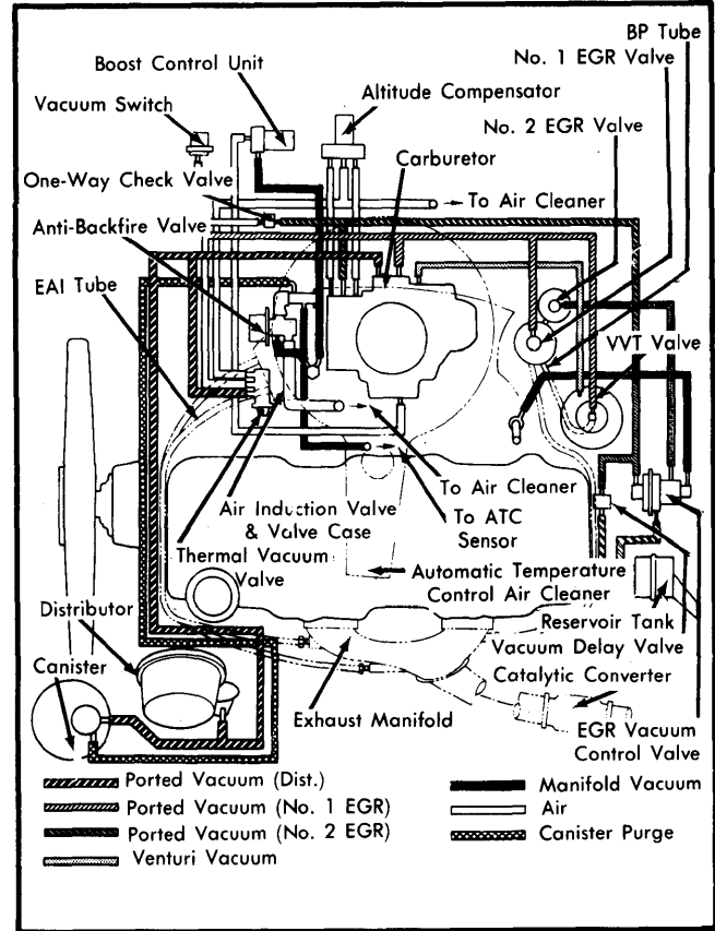
Fig. 3 Datsun 510 Vacuum Diagram (Calif.)
