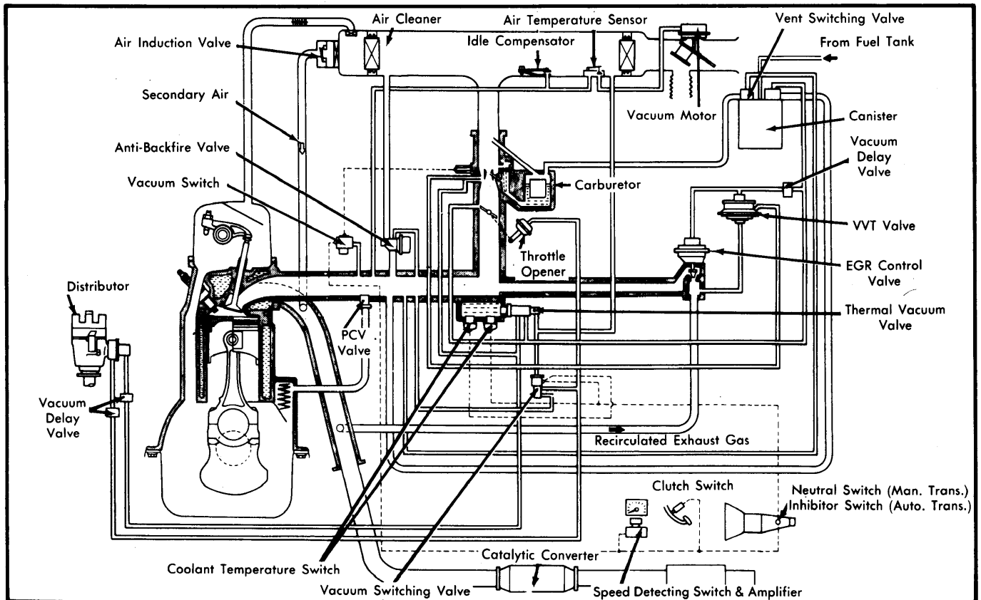
Fig. 7 Datsun 210 Vacuum Diagram (Federal)
