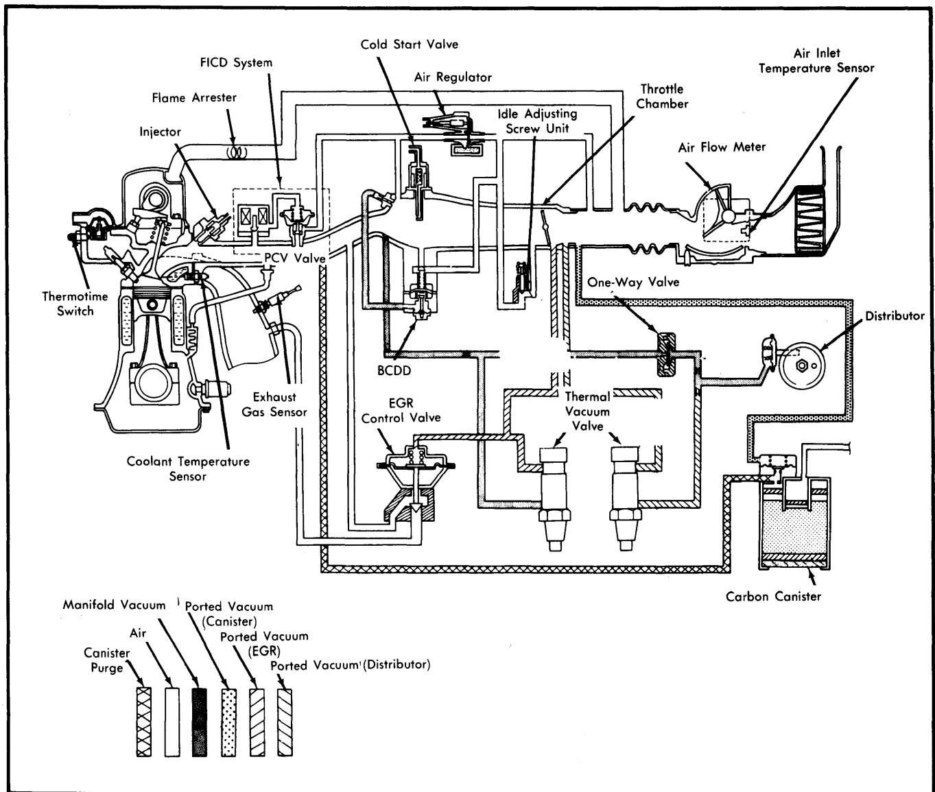
Fig. 10 Datsun 280ZX & 810 Vacuum Diagram
