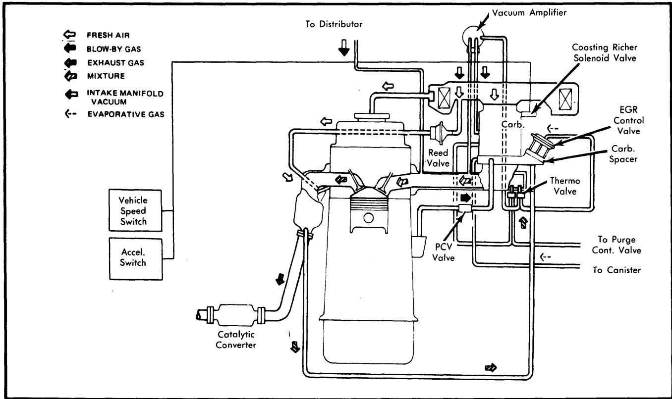
Fig. 3 2.3 Liter Engine Vacuum Diaphragm (Federal Models)
