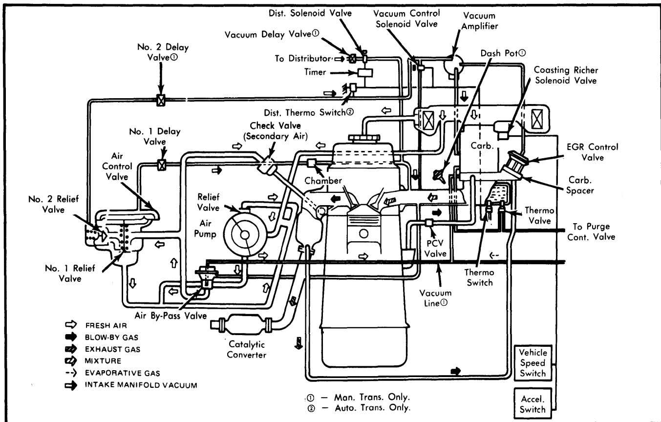
Fig. 4 2.3 Liter Engine Vacuum Diagram (Calif. Models)
