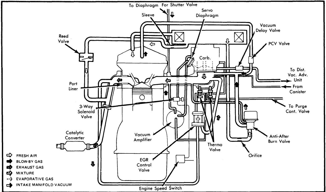
Fig. 1 2.0 Liter Engine Vacuum Diagram (Federal Models)
