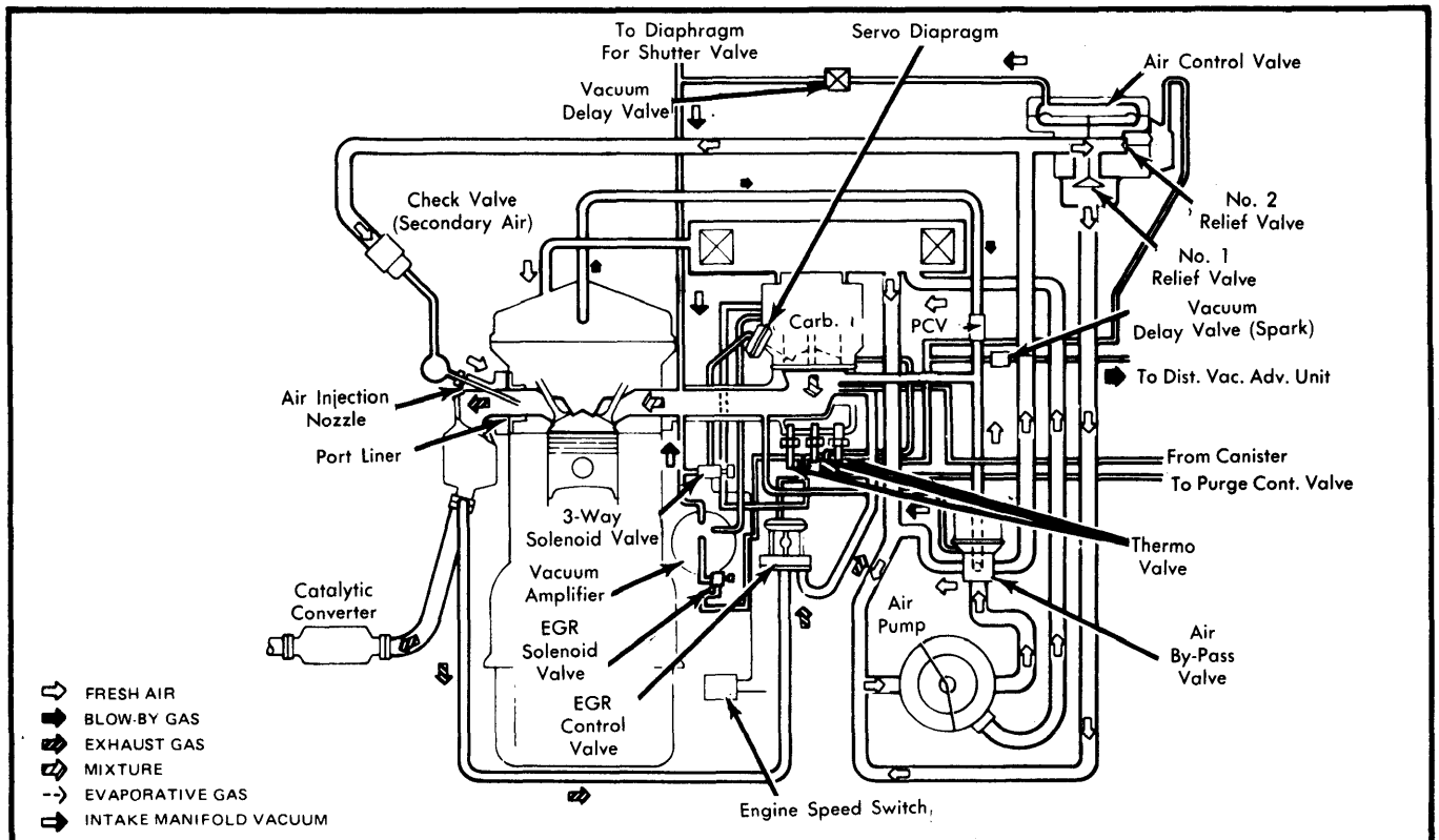
Fig. 2 2.0 Liter Engine Vacuum Diagram (Calif. Models)
