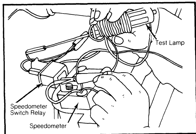
Fig. 4 Testing Speedometer Switch Relay
