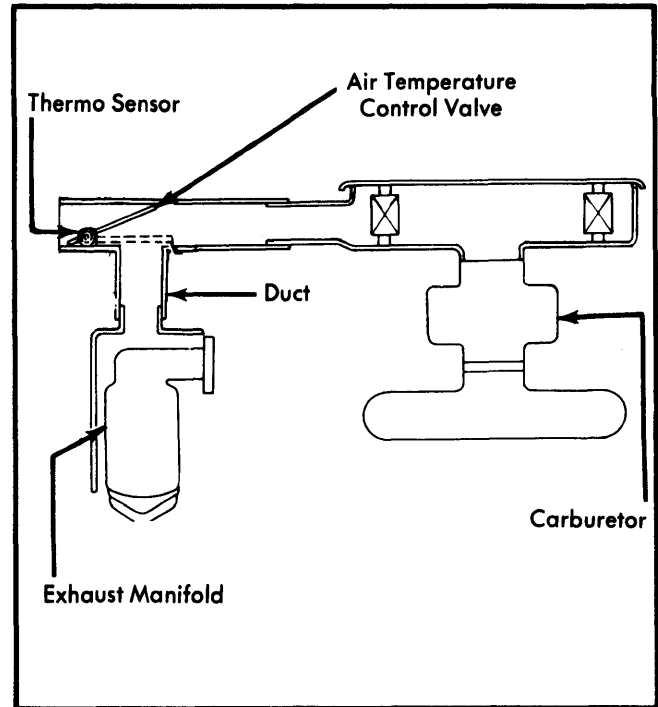
Fig. 1 Courier Thermostatic Air Cleaner Assembly
