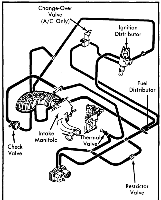
Fig. 4 Audi 5000 Vacuum Diagram (Non-Turbocharged Models)
