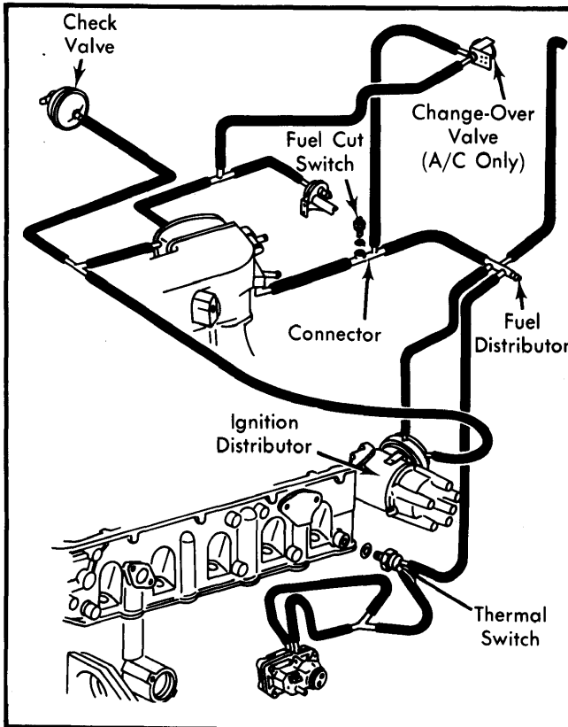
Fig. 3 Audi 5000 Vacuum Diagram (Turbocharged Models)
