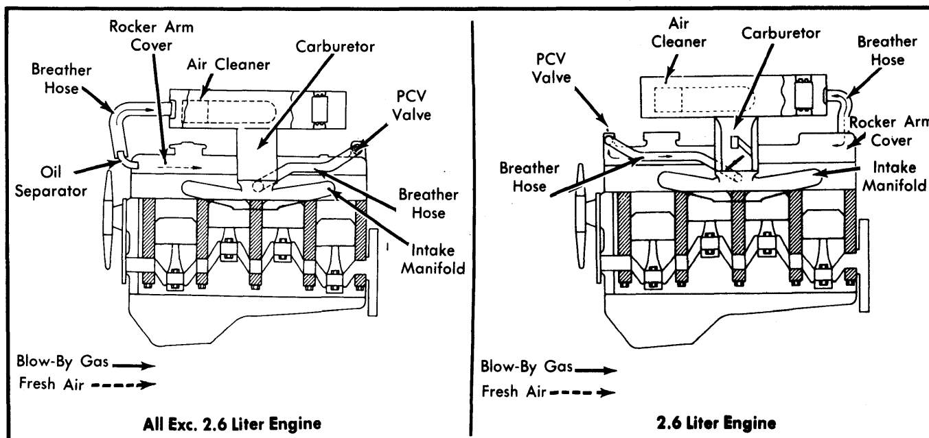
Fig. 1 Chrysler Corp. Imports Crankcase Ventilation System
