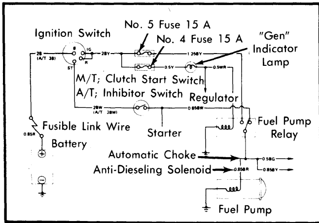
Fig. 1 Isuzu I-Mark Fuel Pump Electrical Circuit
