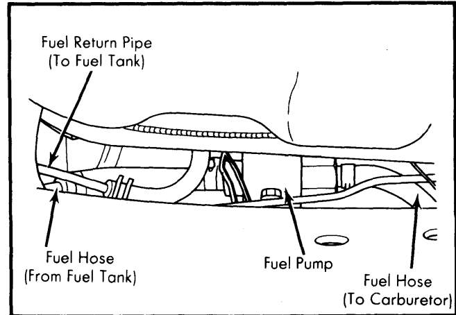
Fig. 3 Typical Fuel Pump Installed Position (Pickup Shown — I-Mark Similar)
