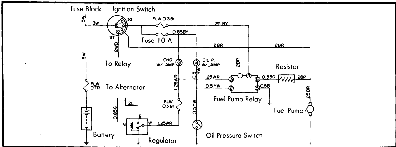
Fig. 2 Isuzu P'UP & LUV Pickup Fuel Pump Electrical Circuit
