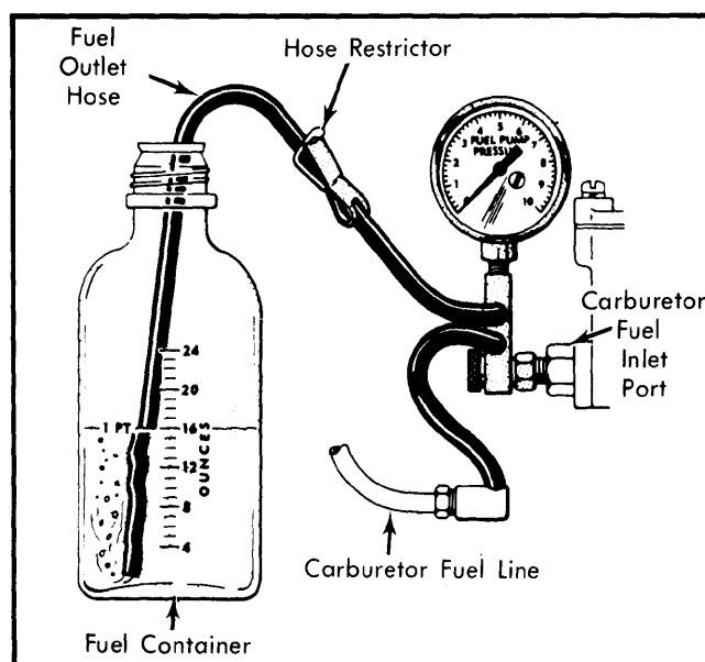
Fig. 2 Fuel Pump Pressure and Volume Test
