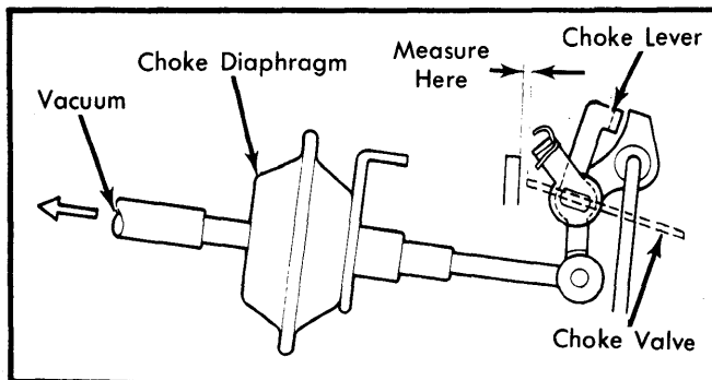
Fig. 6 Adjusting Choke Diaphragm
