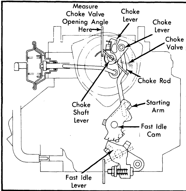
Fig. 5 Adjusting Choke Valve Opening Angle
