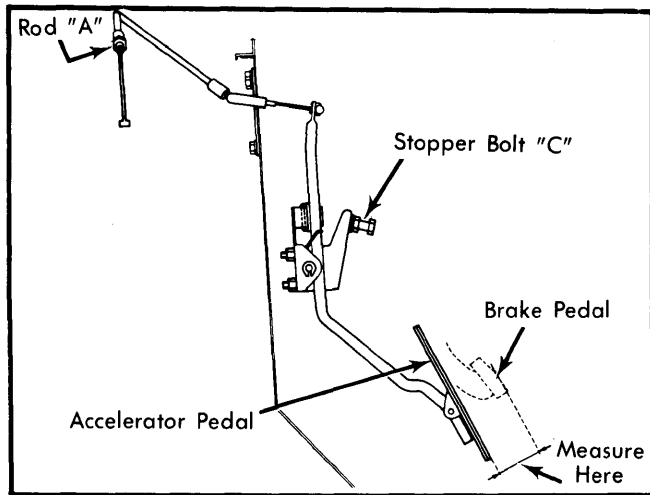
Fig. 9 Adjusting Accelerator Pedal Height
