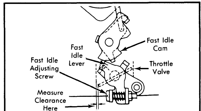
Fig. 4 Choke Linkage Adjustment (Fast Idle Opening Angle)
