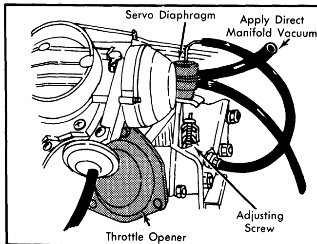
Fig. 10 Adjusting Throttle Opener (A/C Models Only)
