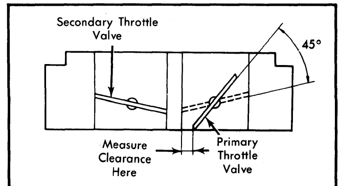
Fig. 8 Adjusting Secondary Throttle Valve Opening Clearance
