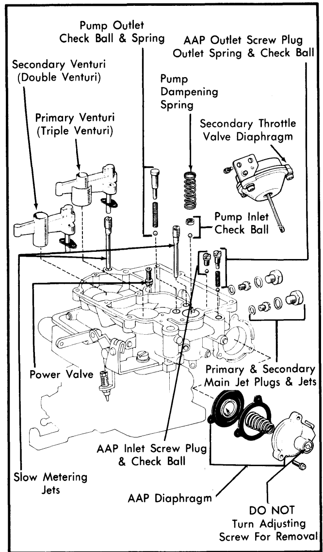
Fig. 9 Exploded View of Carburetor Main Body
