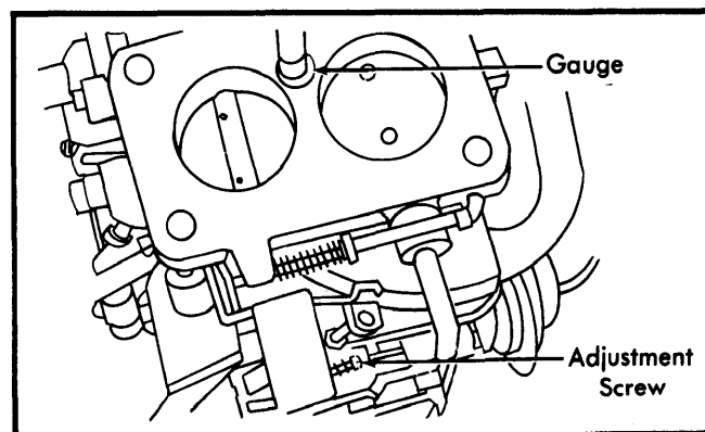
Fig. 3 Making Fast Idle Measurement and Adjustment
