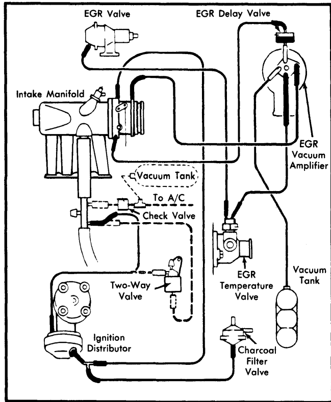
Fig. 1 Vacuum Hose and Emission Control Diagram Federal Dasher, Pickup, Rabbit, Scirocco
