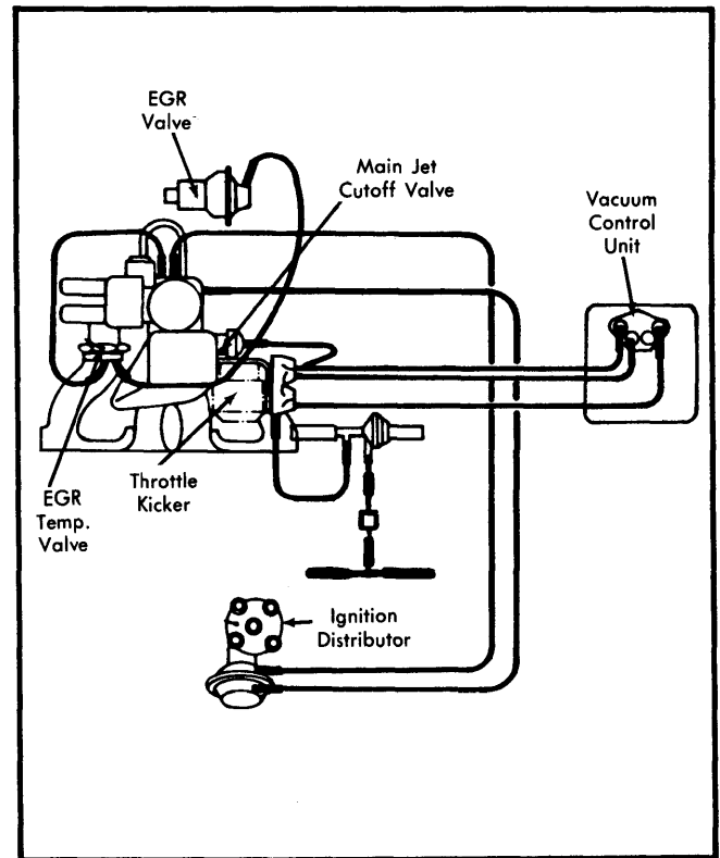
Fig. 2 Vacuum Hose and Emission Control Diagram Federal Rabbit with Carburetor
