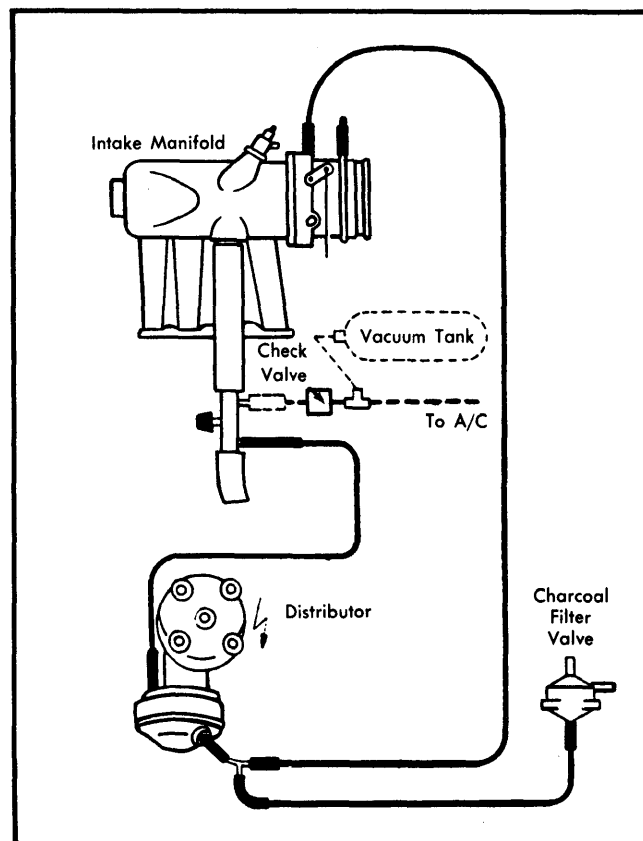
Fig. 3 Vacuum Hose and Emission Control Diagram California Dasher, Pickup, Rabbit, Scirocco
