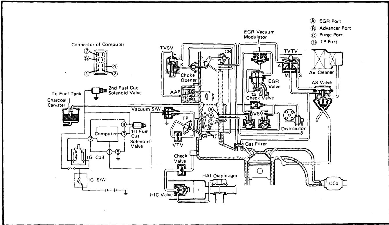
Fig. 1 Toyota Corolla (Federal W/O Cold Advance & High Altitude Compensation)
