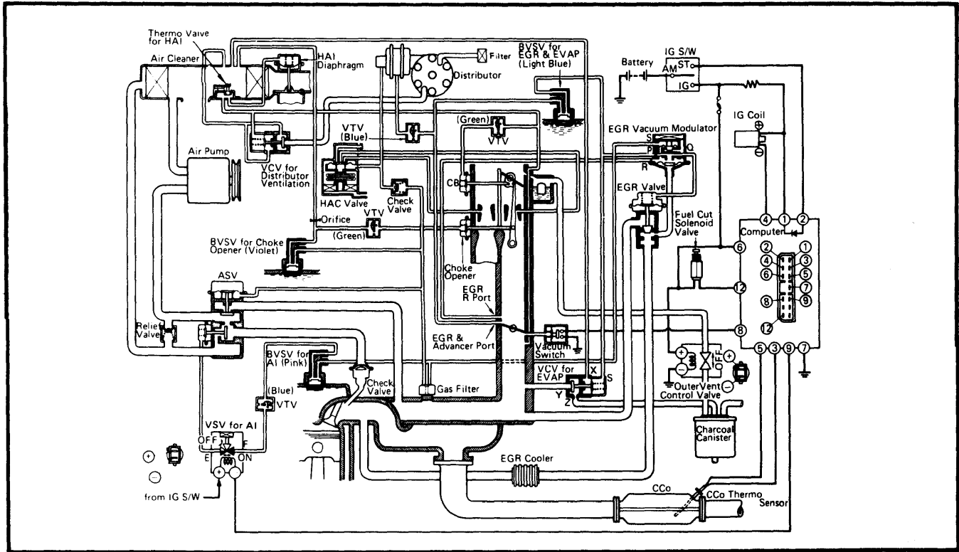
Fig. 13 Toyota Land Cruiser (California)
