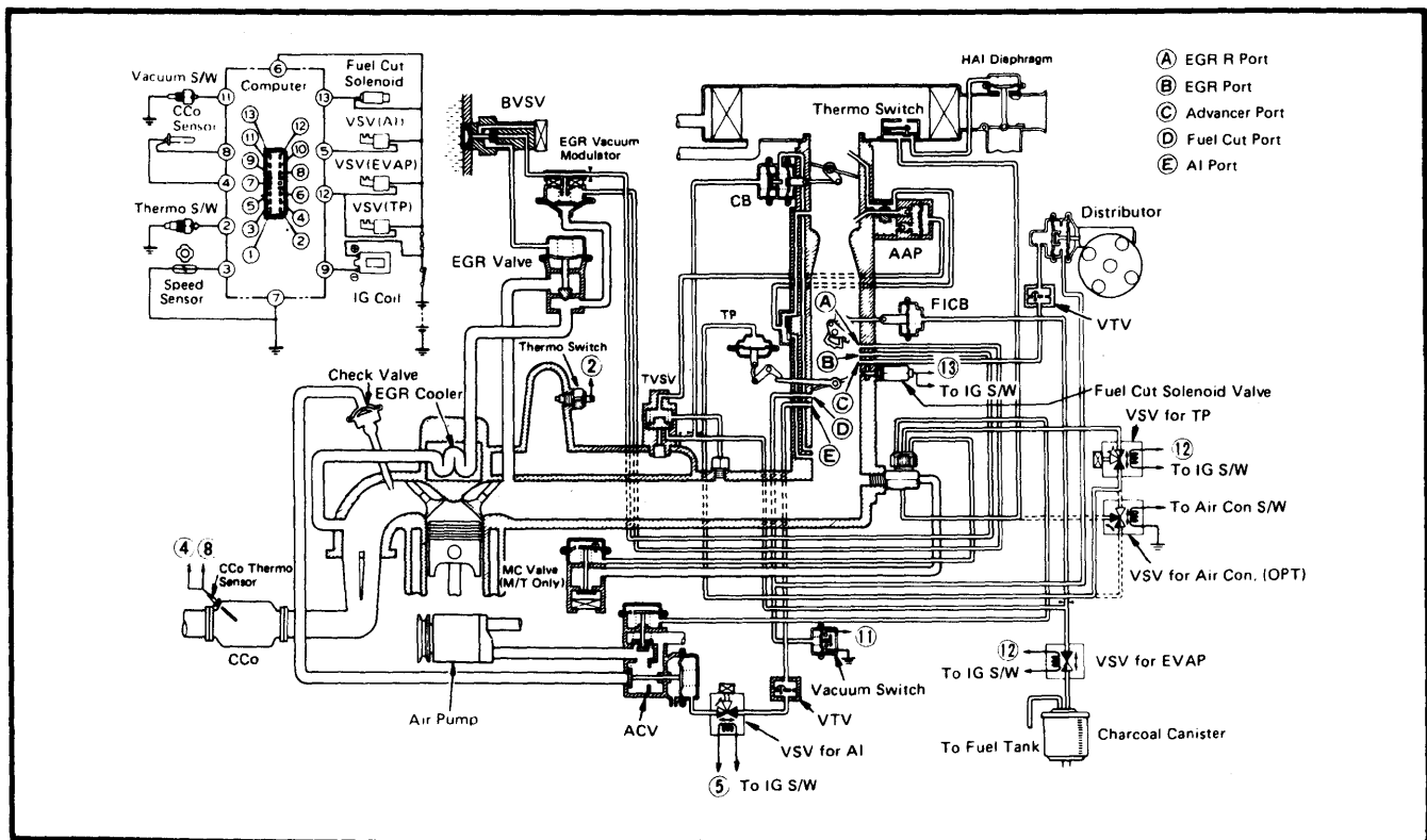
Fig. 6 Toyota Celica and Corona (Federal)
