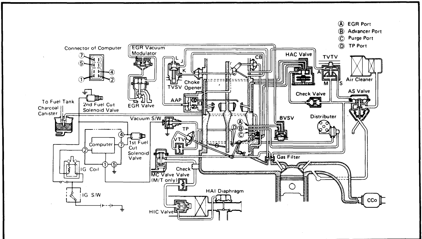
Fig. 3 Toyota Corolla (Federal with High Altitude Compensation)
