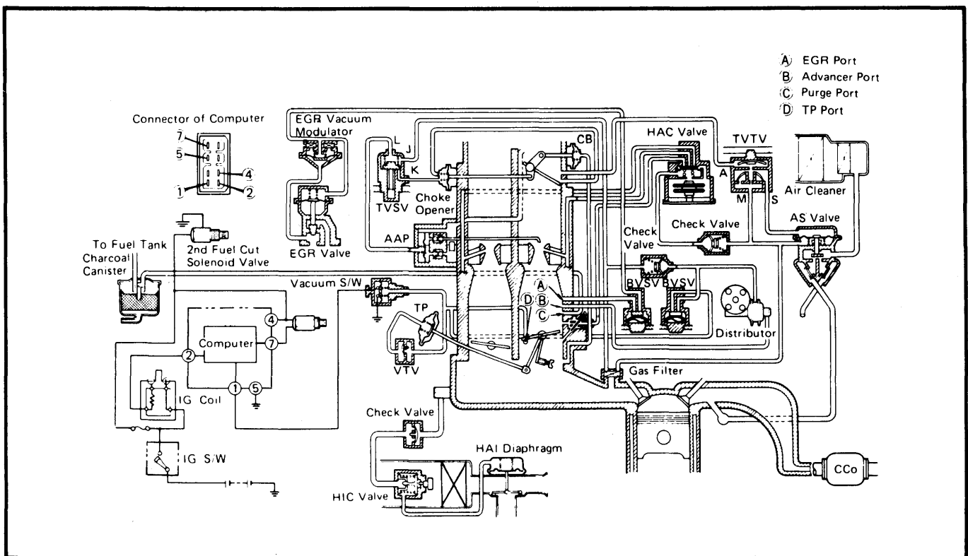
Fig. 4 Toyota Corolla (Federal with Cold Advance and High Altitude Compensation)
