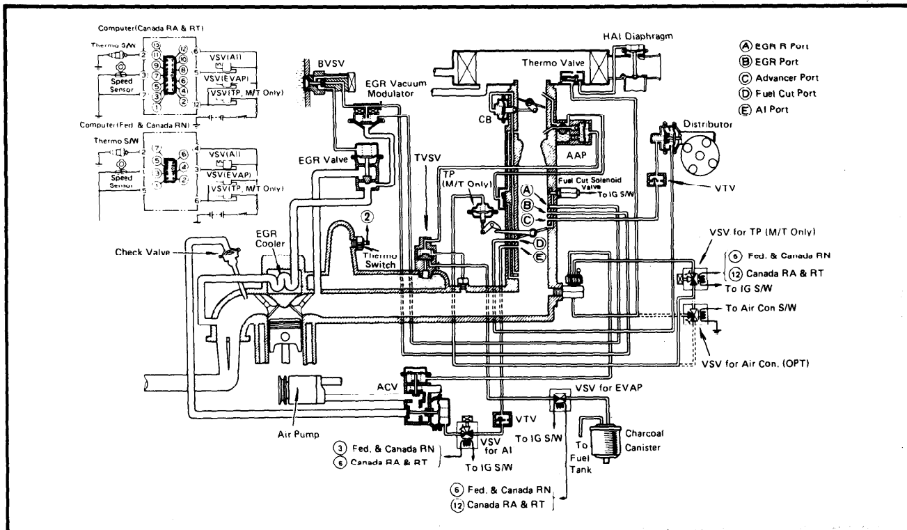
Fig. 7 Toyota Pickup (Federal)
