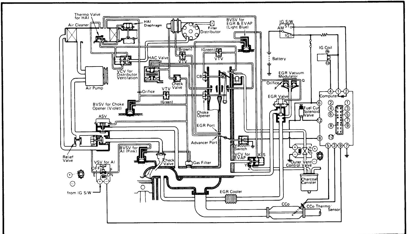
Fig. 12 Toyota Land Cruiser (Federal)
