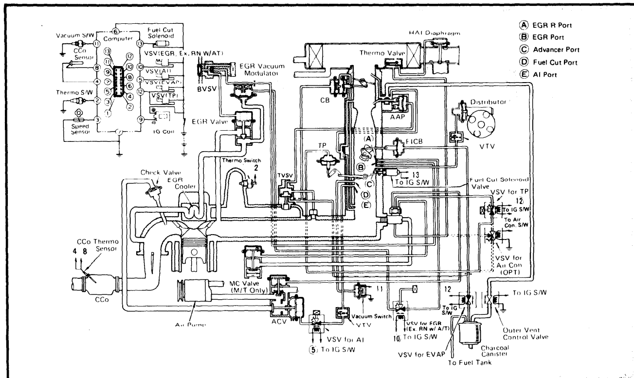
Fig. 8 Toyota Celica, Corona and Pickup (California)
