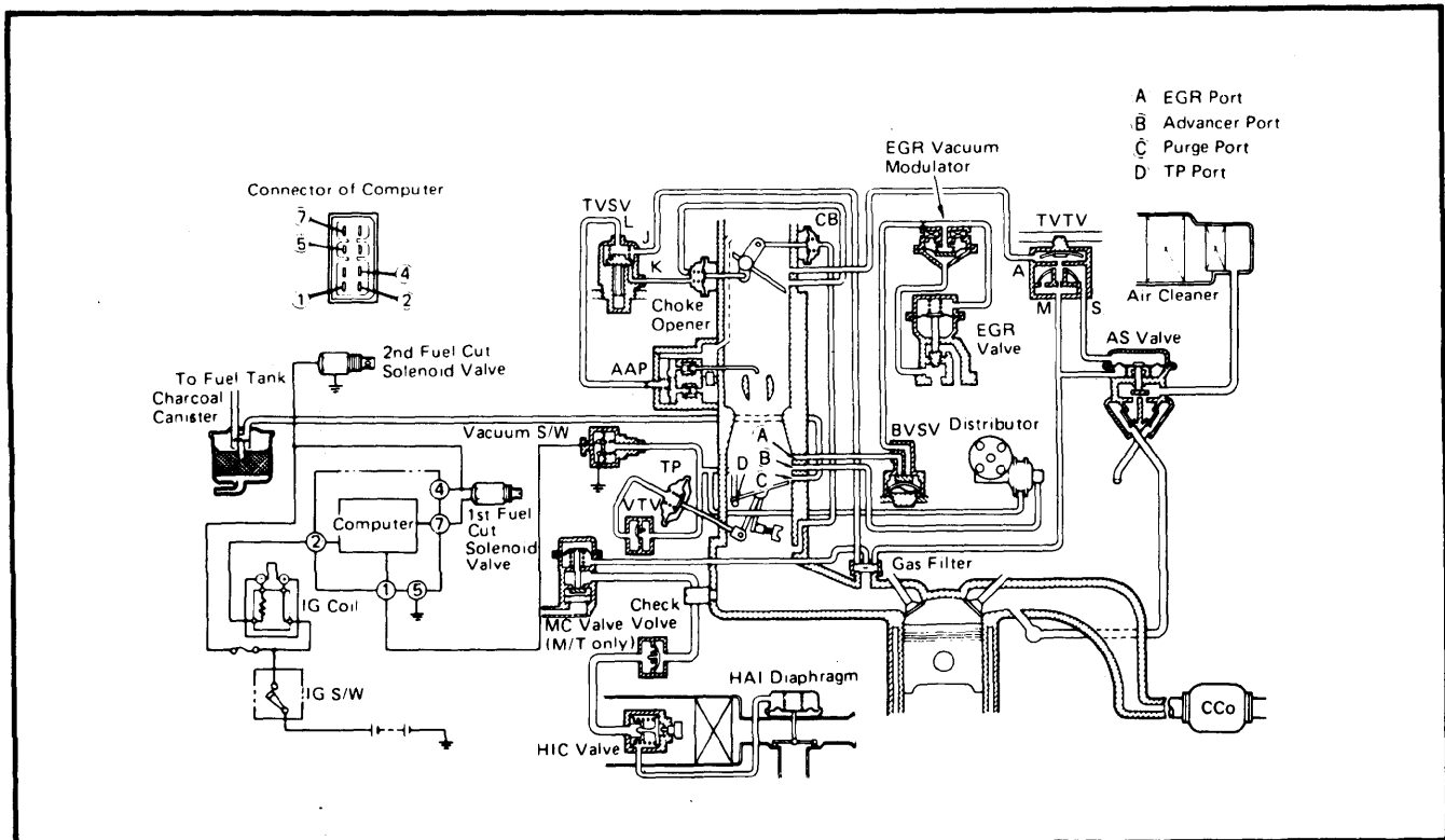
Fig. 2 Toyota Corolla (Federal with Cold Advance System)
