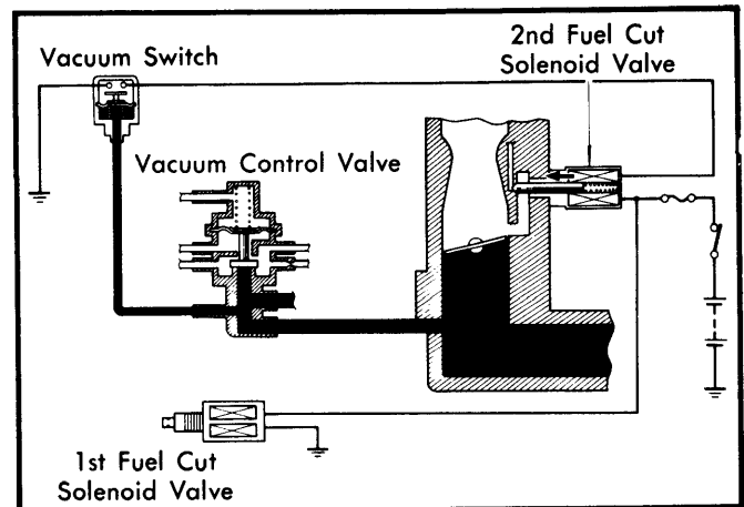
Fig. 2 Tercel Deceleration Fuel Cut System
