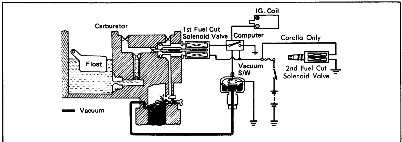
Fig. 1 Schematic of Deceleration Fuel Cut System (All Except Tercel)
