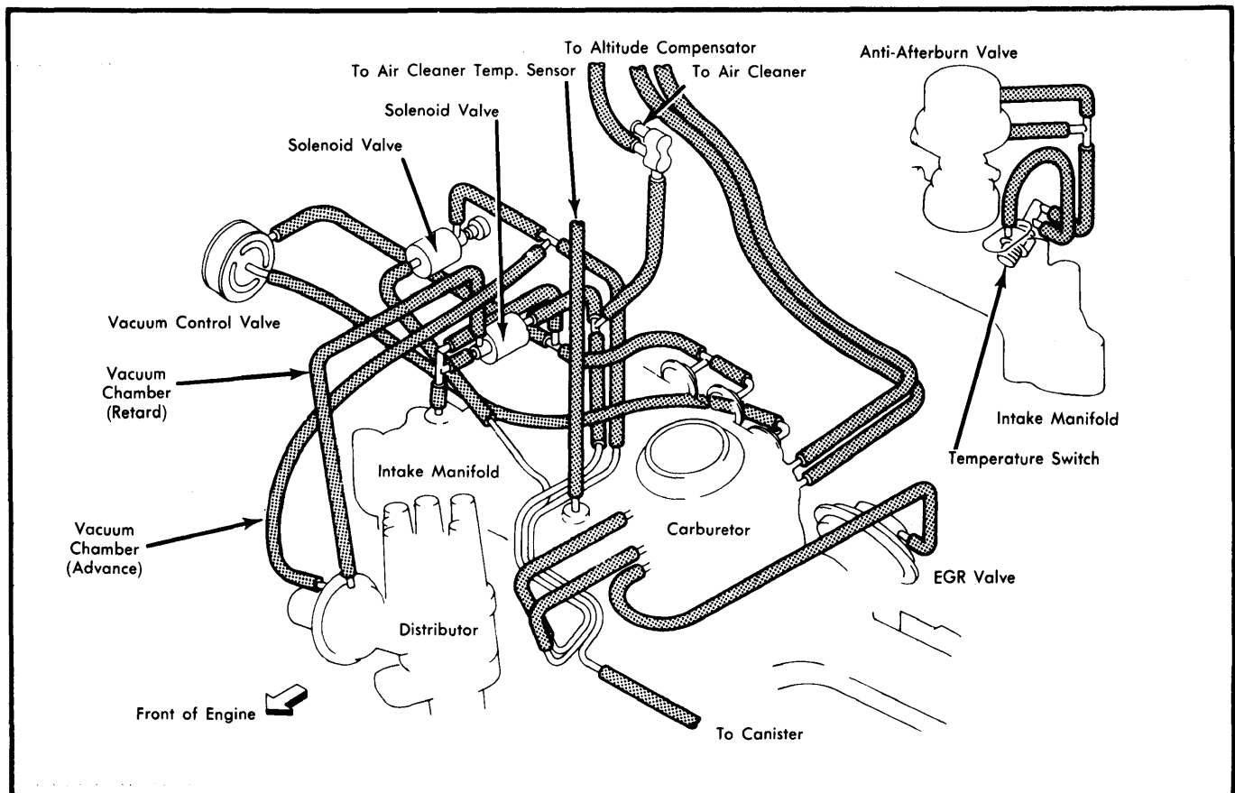
Fig. 4 Calif. 1600 cc Engine With Manual Transmission
