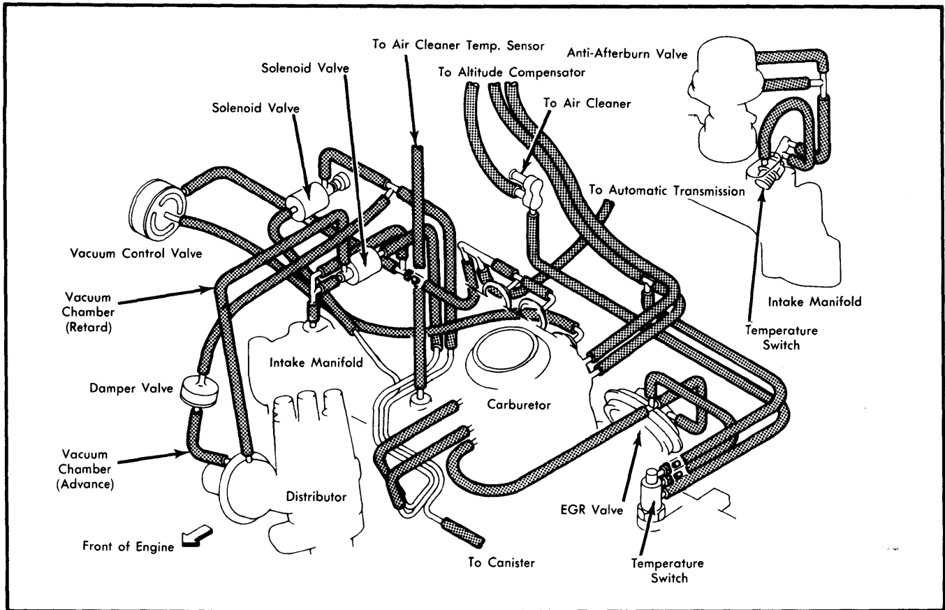
Fig. 5 Calif. 1800 cc Engine With Automatic Transmission
