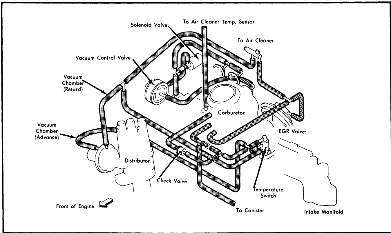
Fig. 2 Federal 1600 cc Engine With Manual Transmission (Hatchback, Sedan DL and Hardtop DL)
