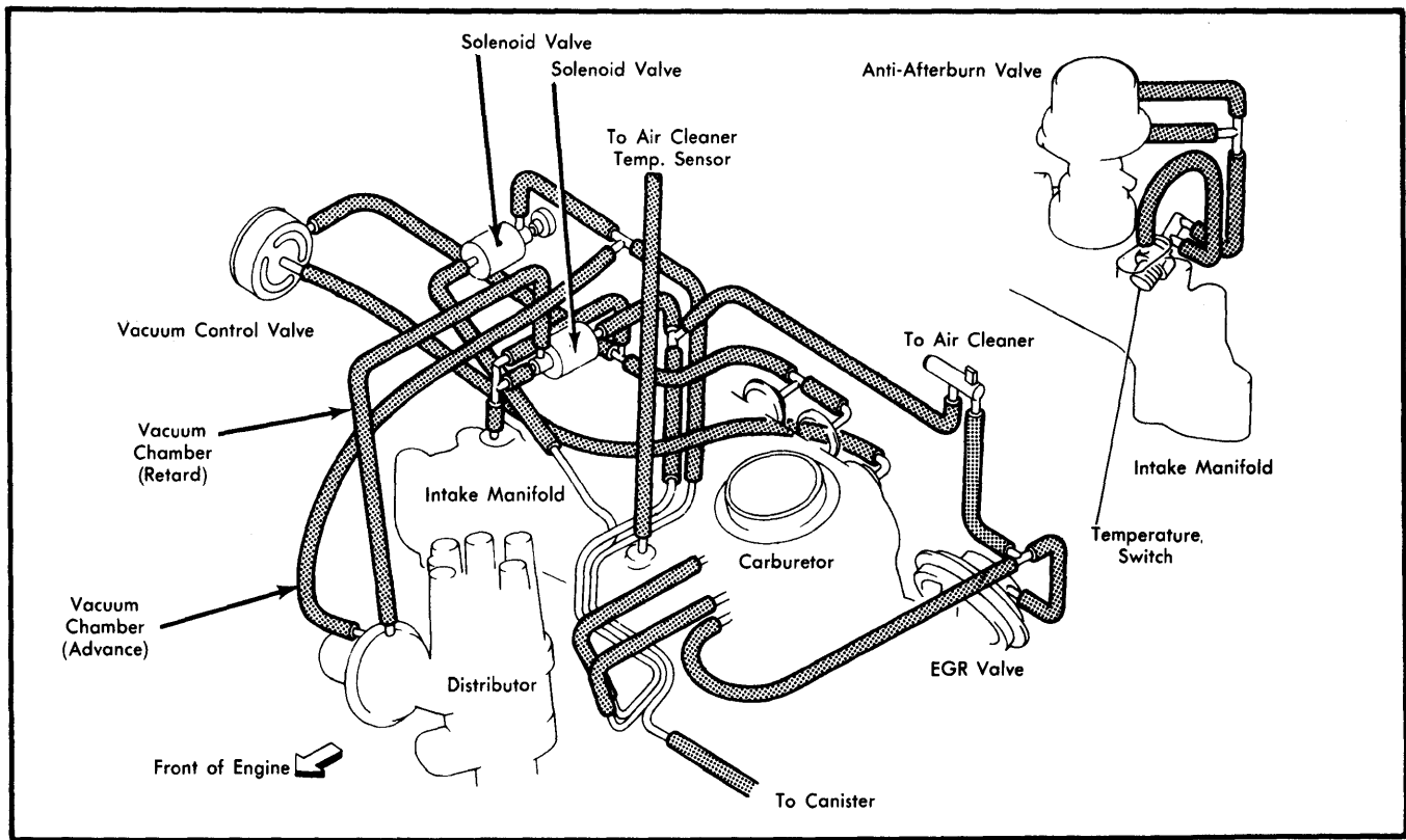
Fig. 1 Federal 1600 cc Engine With Manual Transmission (Exc. Hatchback, Sedan DL and Hardtop DL)
