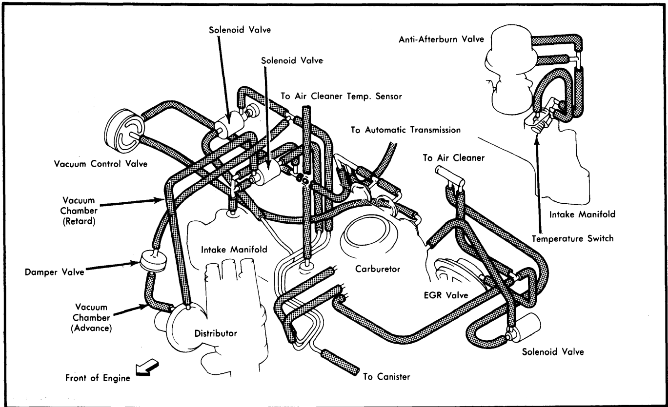
Fig. 3 Federal 1800 cc Engine With Automatic Transmission
