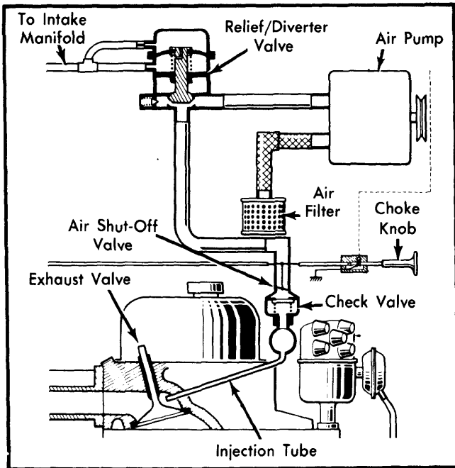
Fig. 1 Le Car Air Injection System
