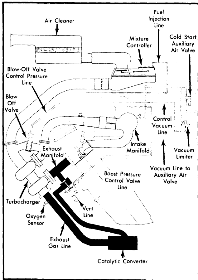
Fig. 3 Porsche 924 Turbo Vacuum Diagram
