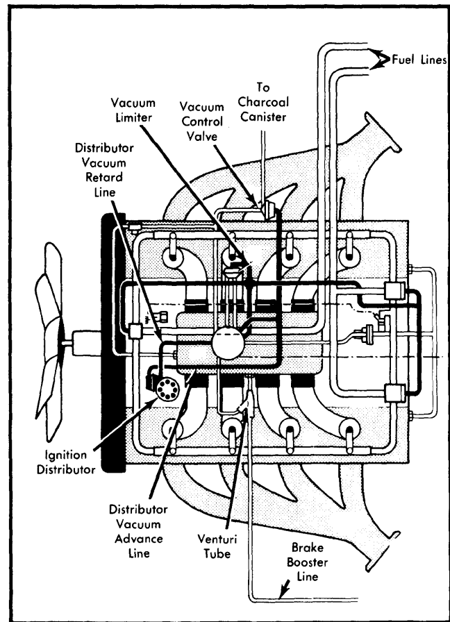
Fig. 4 Porsche 928 Vacuum Diagram
