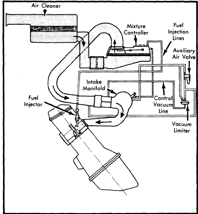
Fig. 2 Porsche 924 Vacuum Diagram
