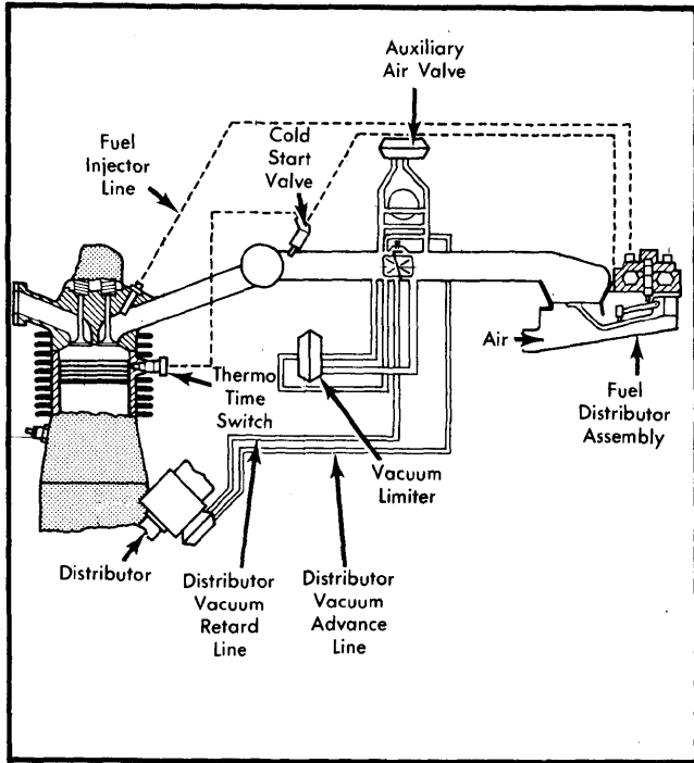
Fig. 1 Porsche 911 SC Vacuum Diagram
