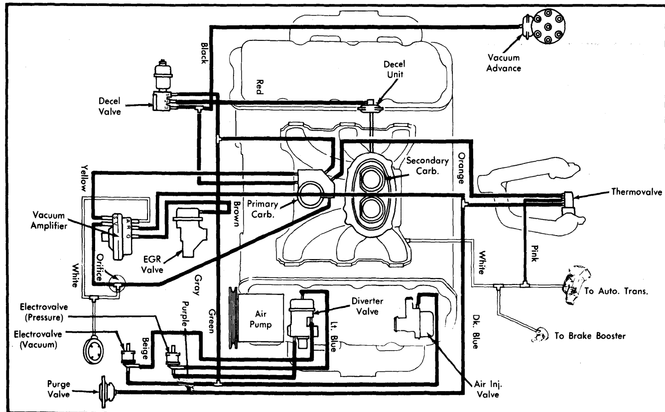
Fig. 2 604 Automatic Transmission Vacuum Hose Diagram
