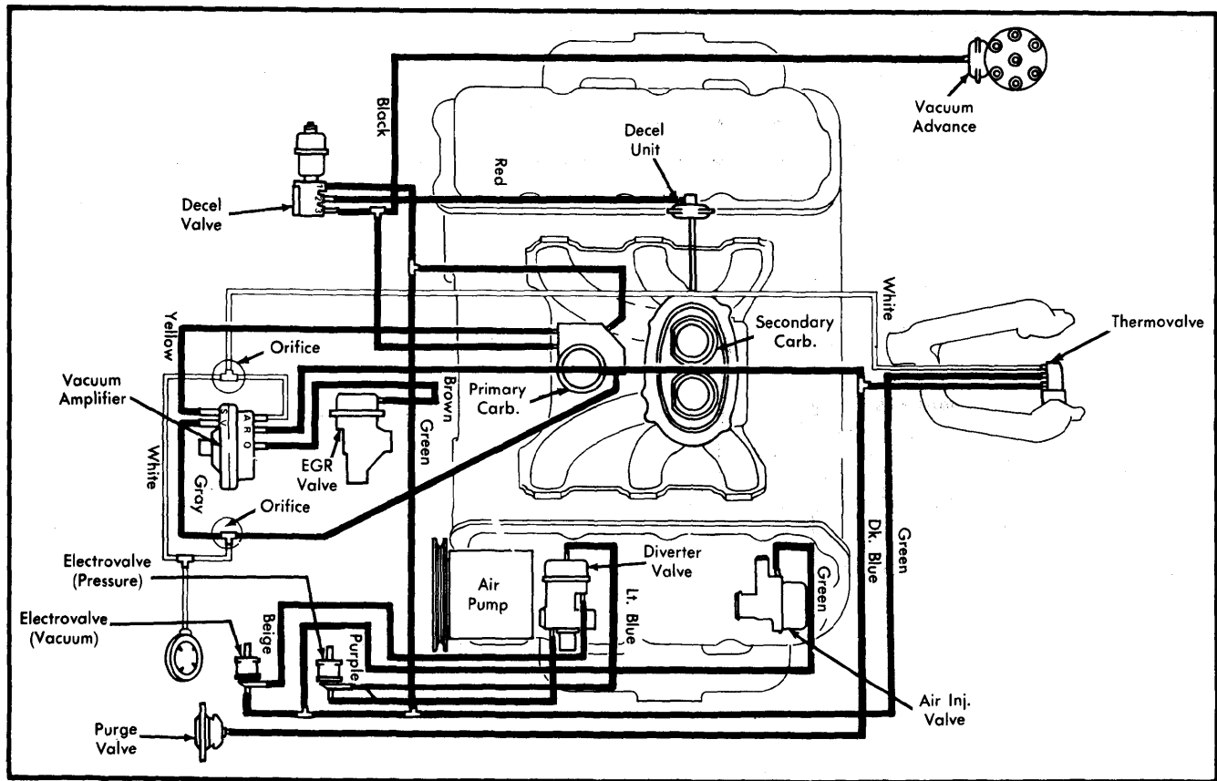
Fig. 1 604 Manual Transmission Vacuum Hose Diagram
