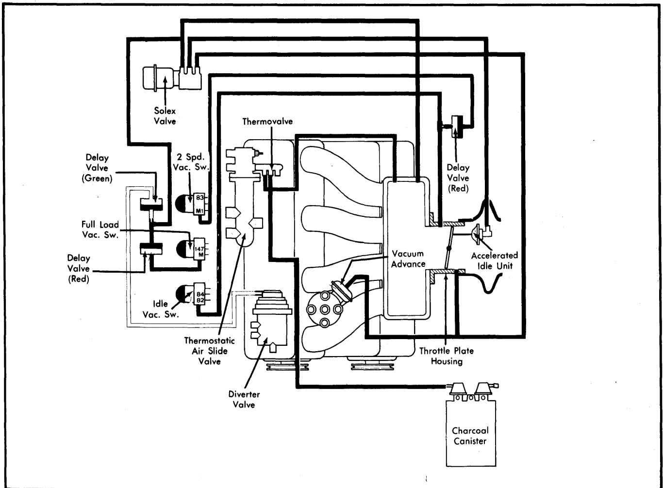
Fig. 3 505 Vacuum Hose Diagram
