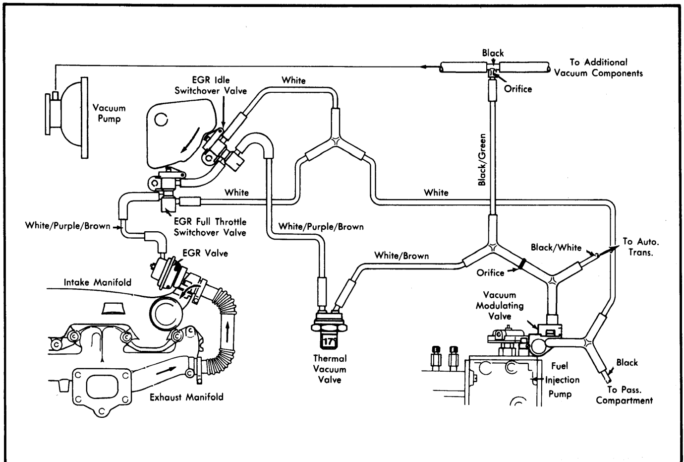
Fig. 4 300 SD Turbo Emission Control Vacuum Hose Routing
