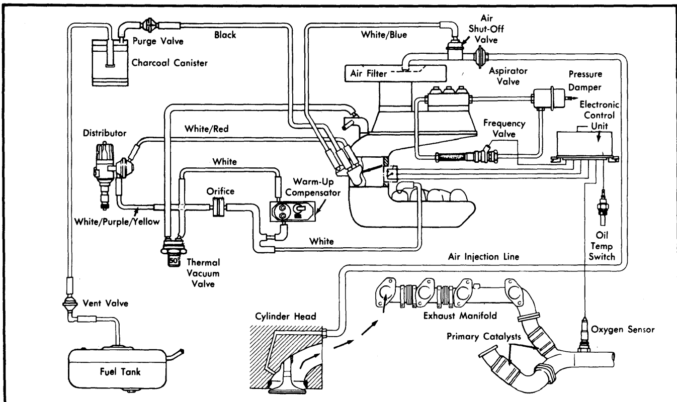
Fig. 2 450 Series Emission Control Vacuum Hose Routing
