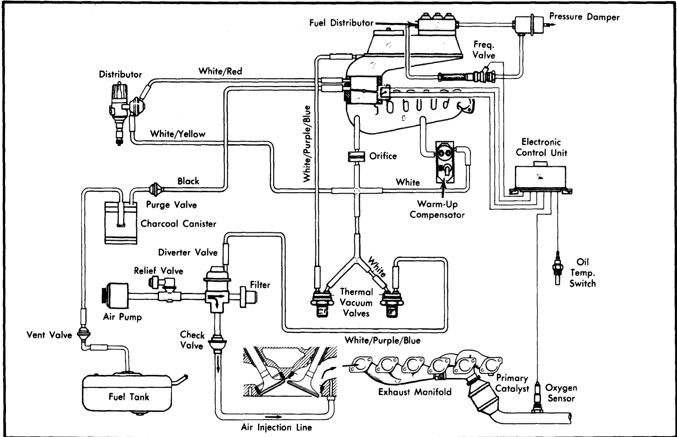
Fig. 1 280 Series Emission Control Vacuum Hose Routing
