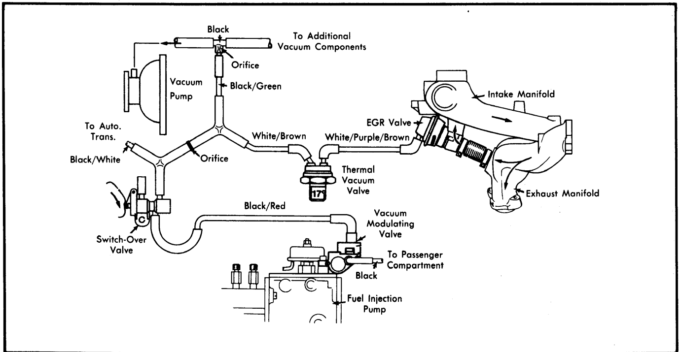
Fig. 3 300 Series Emission Control Vacuum Hose Routing (Except 300SD Turbo)
