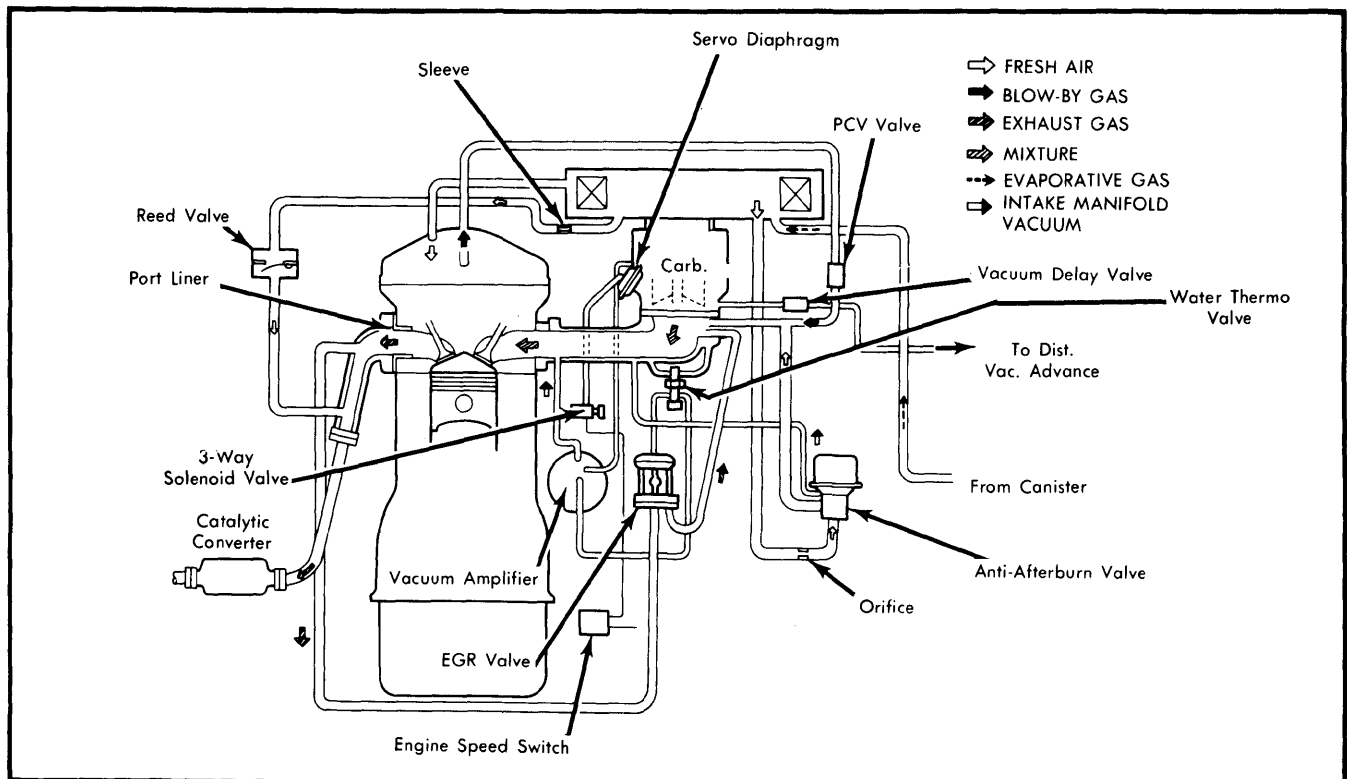
Fig. 4 Vacuum Hose Routing for Mazda B2000 (Federal, All Trans.)
