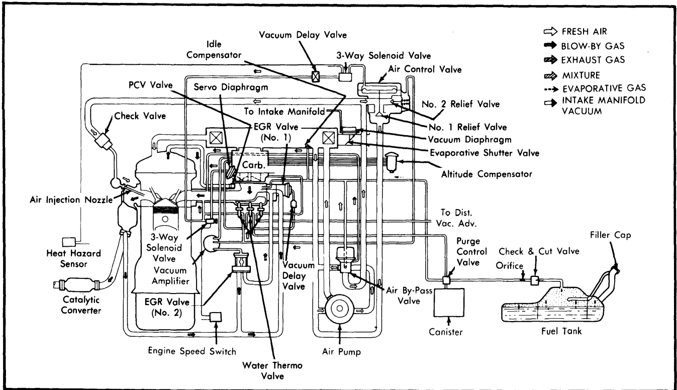
Fig. 3 Vacuum Hose Routing for Mazda 626 (All Models, All Trans.)
