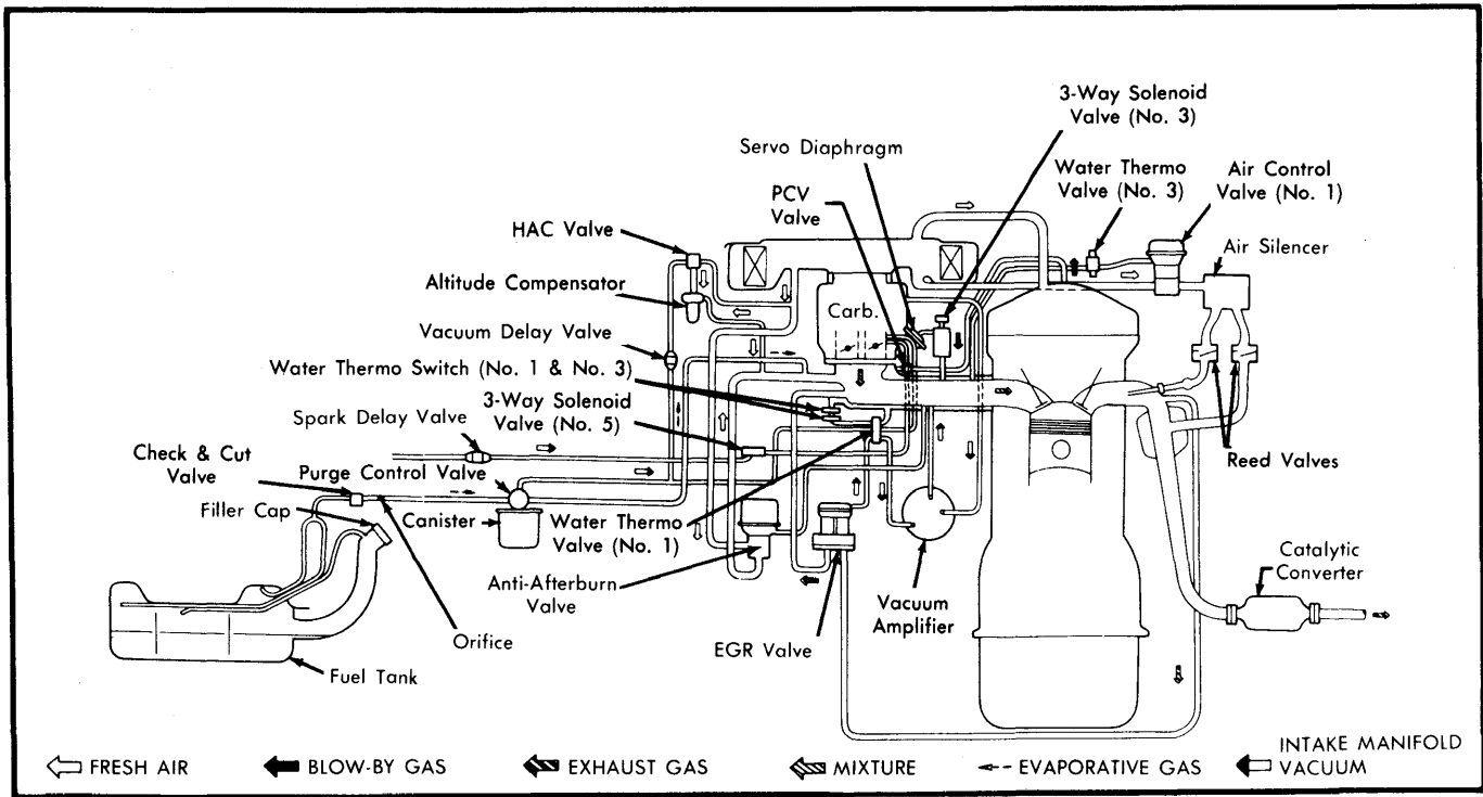
Fig. 1 Vacuum Hose Routing for Mazda GLC (All Exc. Calif. with Auto. Trans.)
