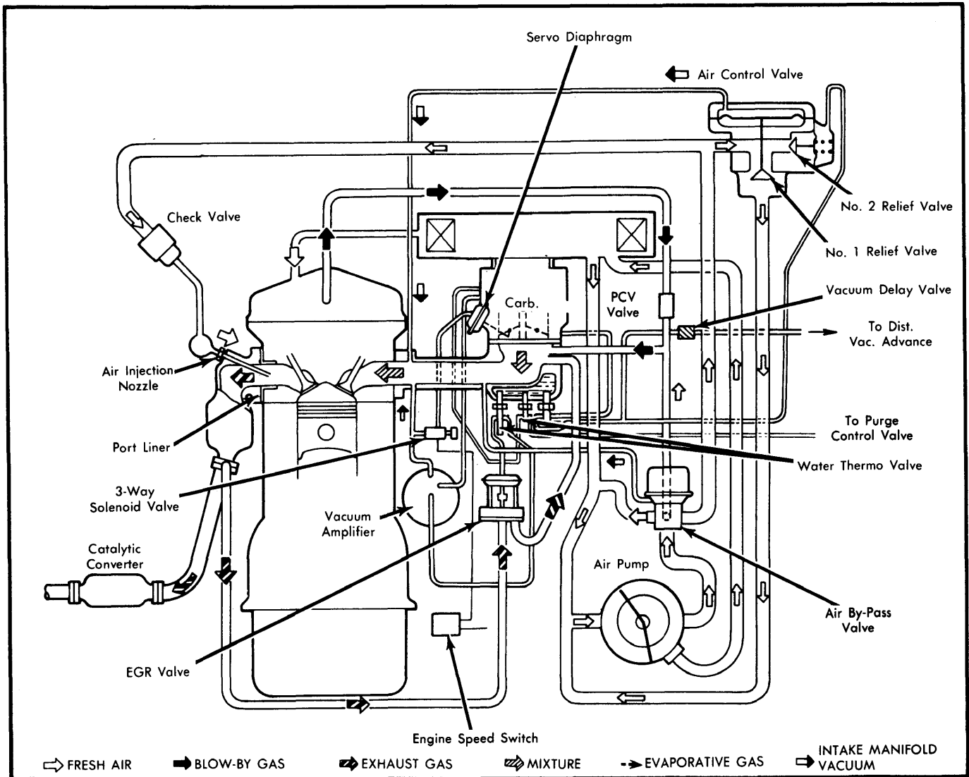
Fig. 5 Vacuum Hose Routing for Mazda B2000 (Calif., All Trans.)
