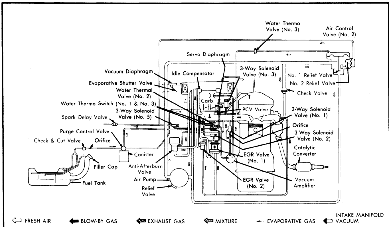
Fig. 2 Vacuum Hose Routing for Mazda GLC (Calif. with Auto. Trans.)
