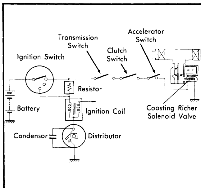
Fig. 1 LUV Coasting Richer System Schematic (Federal Man. Trans. Vehicles)
