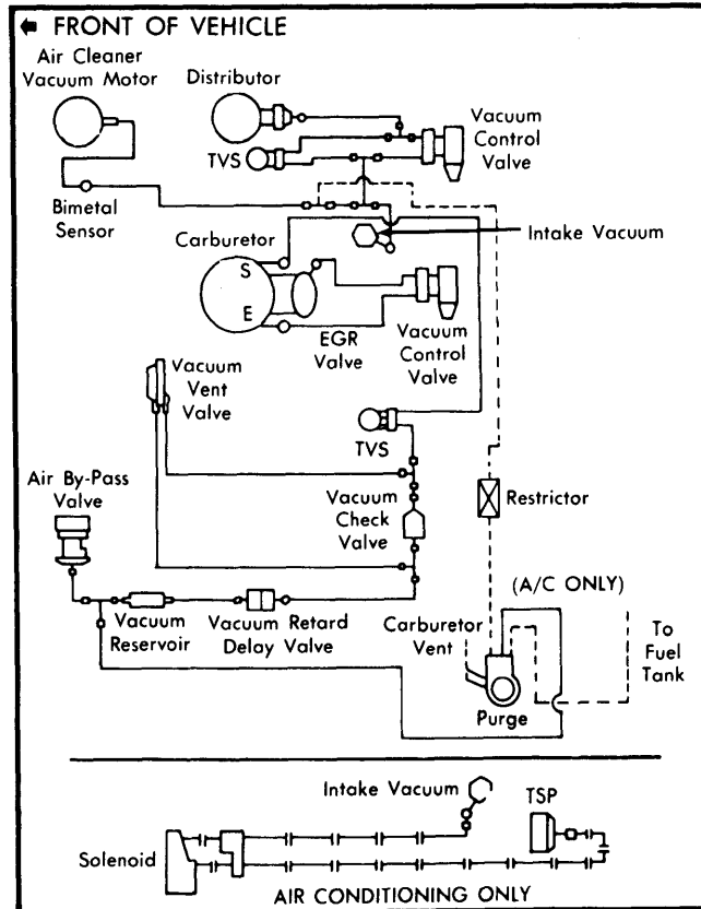
Fig. 3 Fiesta Emission Control Vacuum Diagram (California Calibration No. 0-5N-RO)
