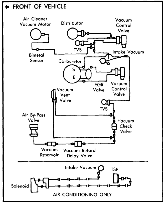
Fig. 2 Fiesta Emission Control Vacuum Diagram (Federal Calibration No. 0-5B-R2)
