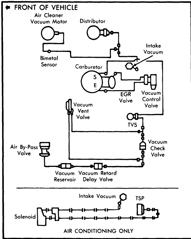
Fig. 1 Fiesta Emission Control Vacuum Diagram (Federal Calibration No. 0-5B-R1)
