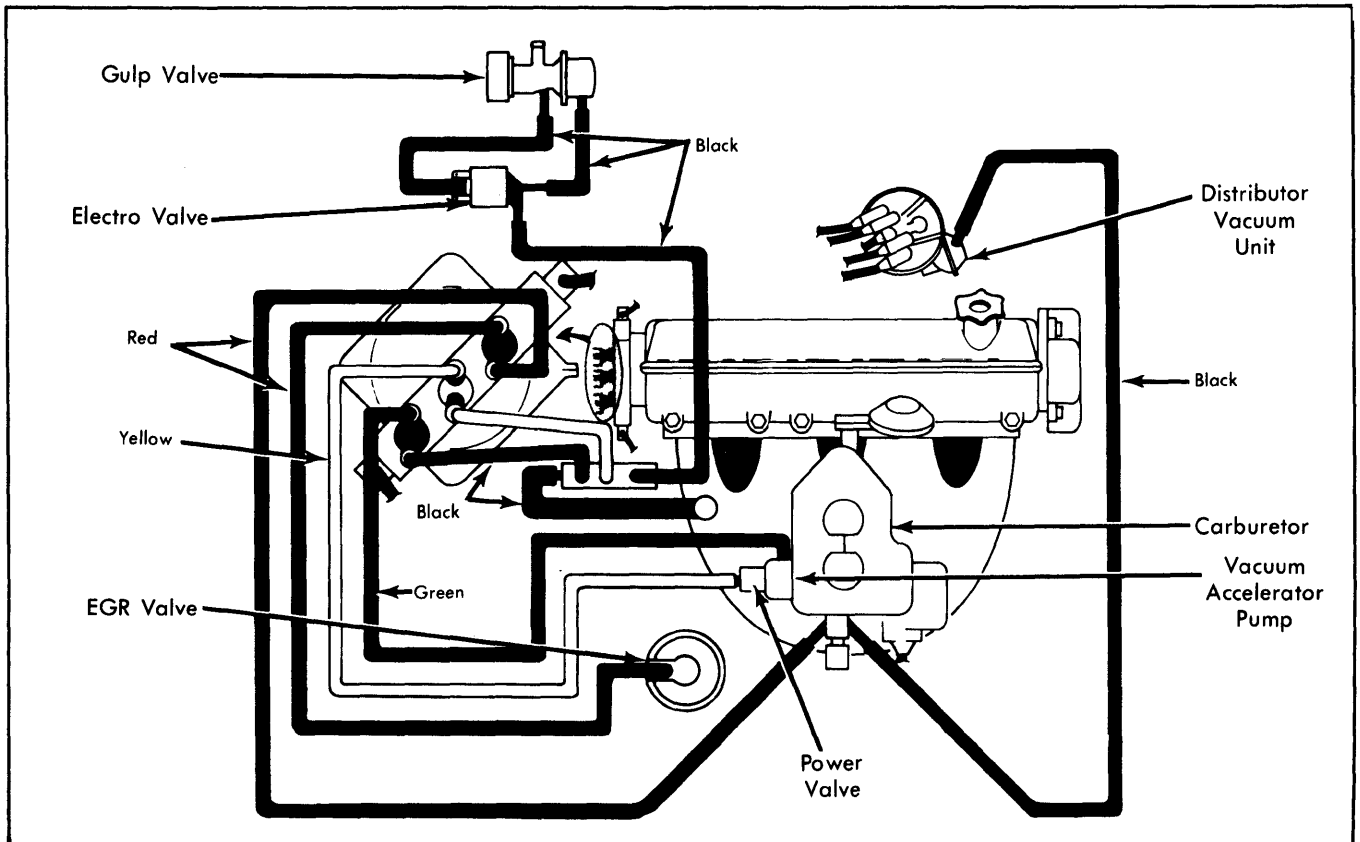
Fig. 2 Strada and X1/9 Carbureted Models Vacuum Diagram
