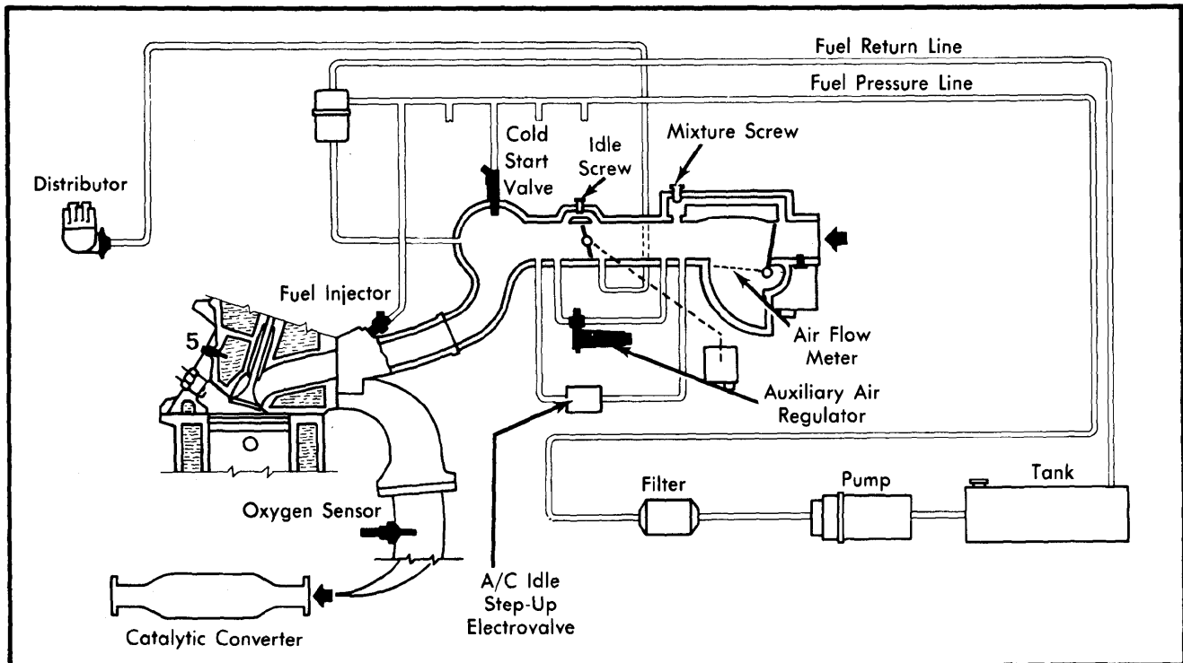
Fig. 4 Strada and X1/9 Fuel Injected Models Emission Control Diagram
