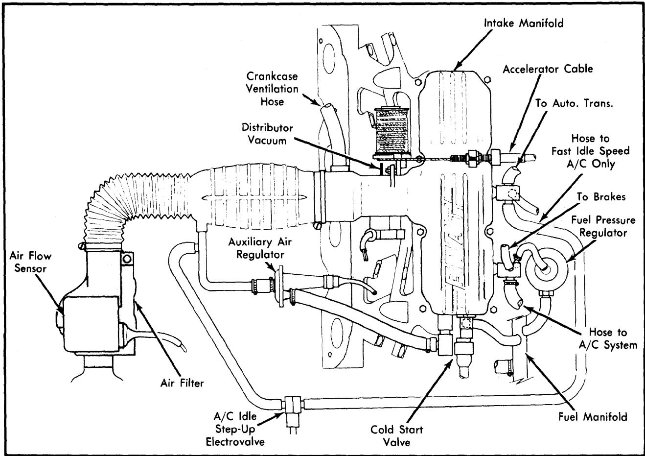
Fig. 3 Brava and Spider 2000 Fuel Injected Models Vacuum Diagram
