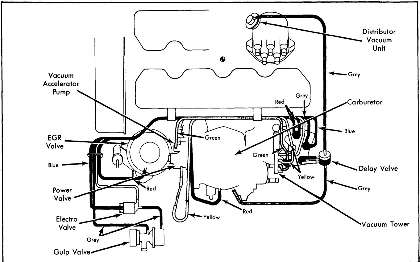
Fig. 1 Brava and Spider 2000 Carbureted Models Vacuum Diagram
