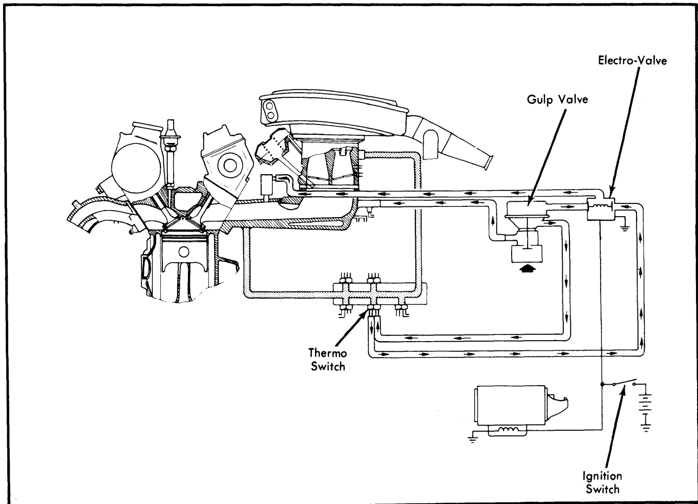
Fig. 1 Fiat Air Gulp System (Brava and Spider Models Shown - Strada and X1/9 Models Similar)
